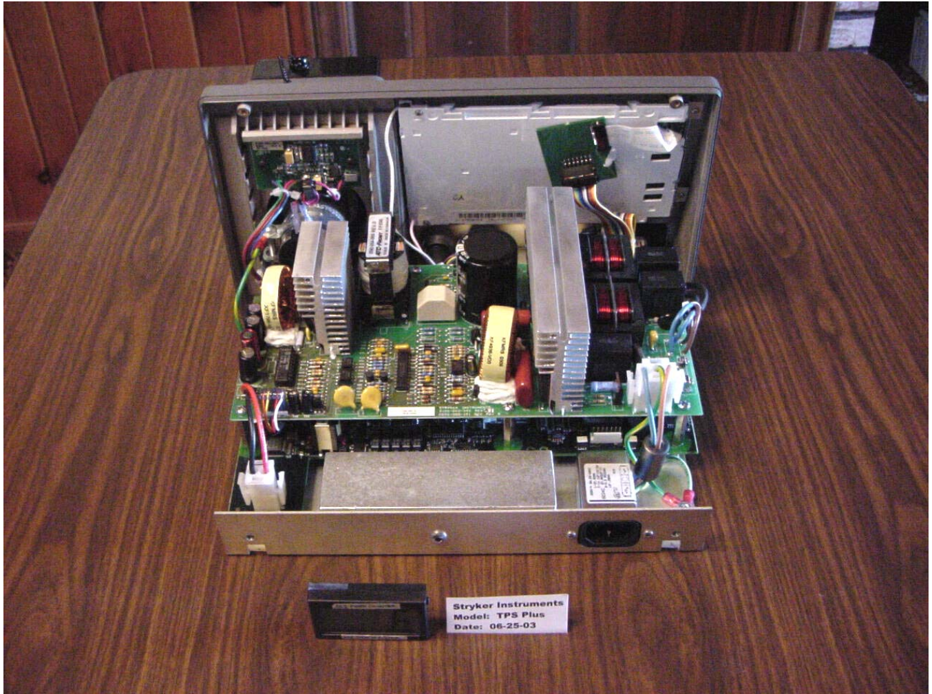
BACK COVER OF TPS IRRIGATION CONSOLE REMOVED
