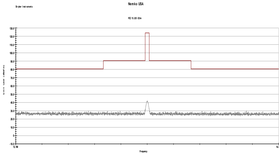
Figure 8.3-2: Field strength within 13.11–14.010 MHz band
