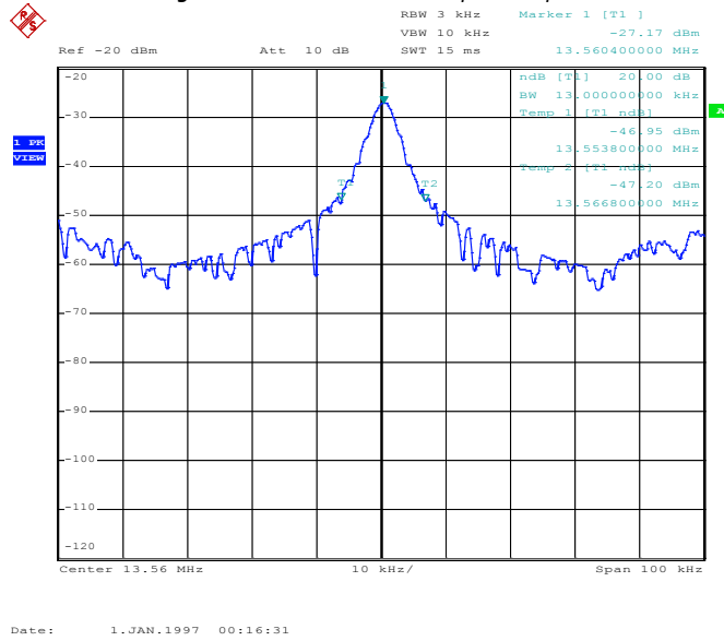
Figure 8.1-1: 20 dB bandwidth spectrum plot
