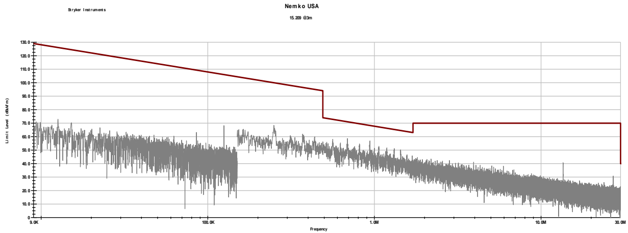
Figure 8.4-1: Field strength of spurious emissions below 30 MHz
