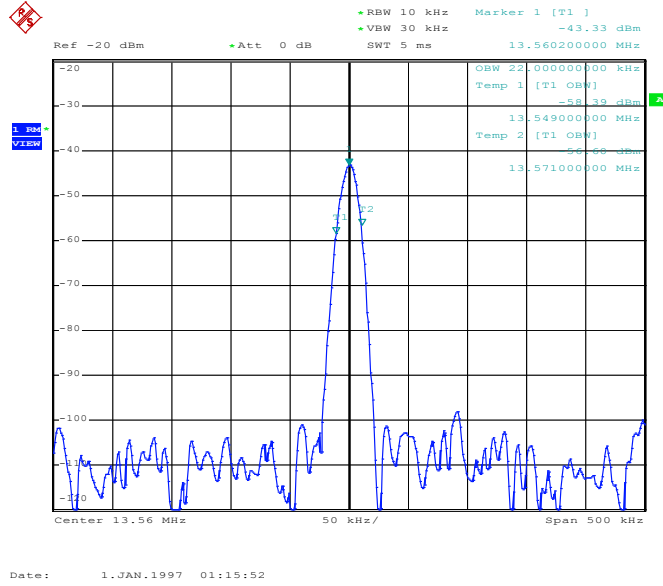
Figure 8.2-1: 99 % occupied bandwidth
