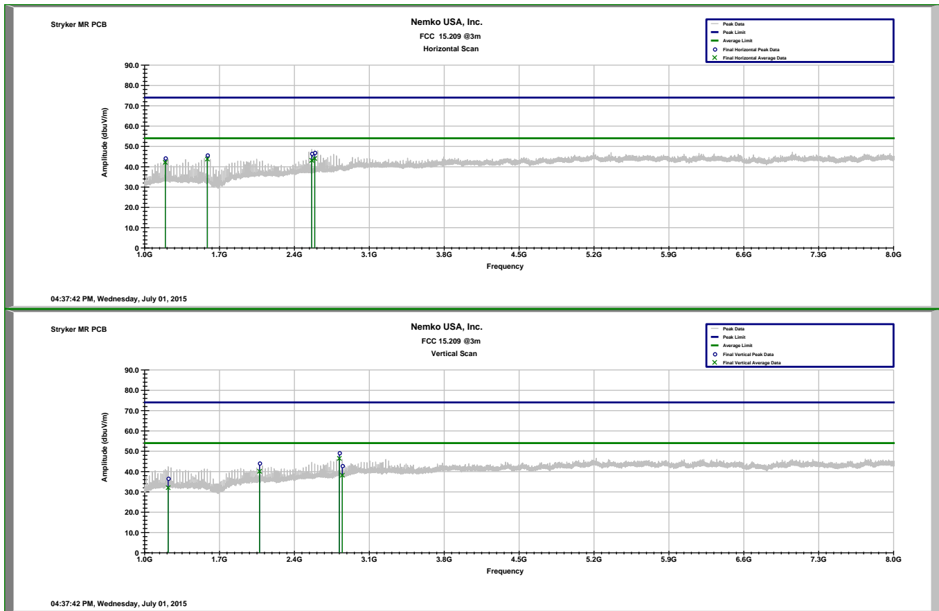
Figure 8.4-3: Field strength of spurious emissions 1-8GHz
