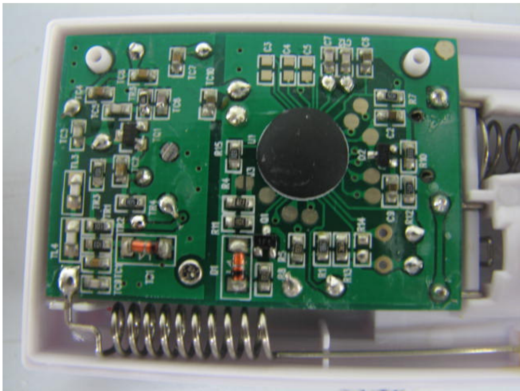
Transmitter
