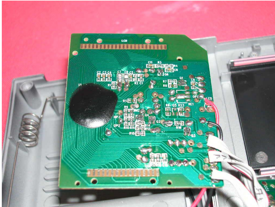
Internal Photo – 8
