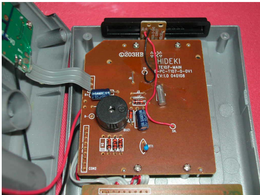
Internal Photo – 2
