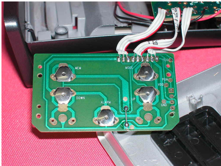
Internal Photo – 8
