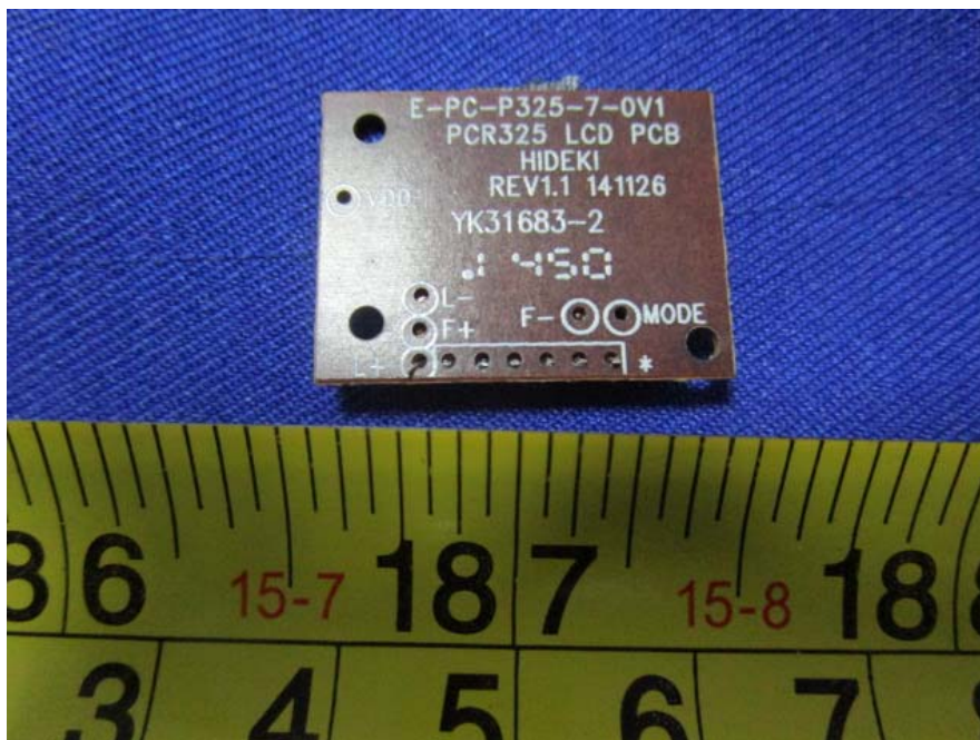
EUT –EUT –Subboard 1 Bottom View
