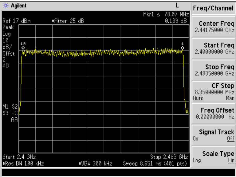
8DPSK Modulation
