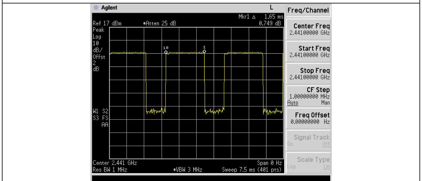
2-DH3
