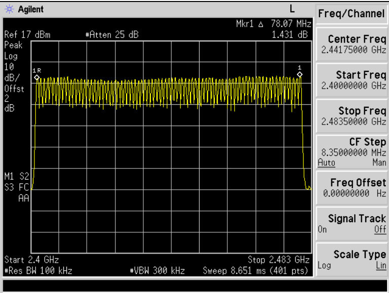
GFSK Modulation
