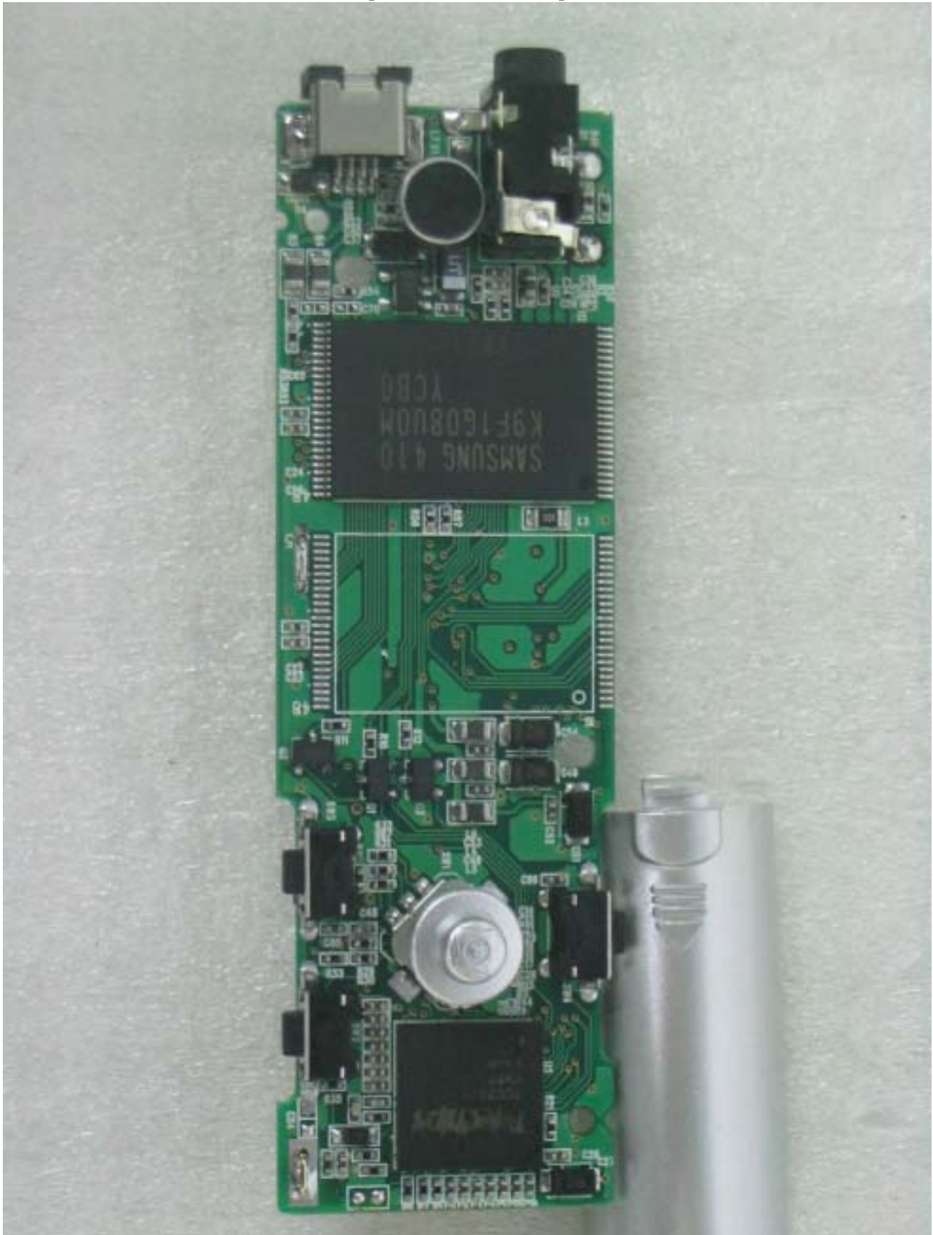
[Bottom of PCB side]
