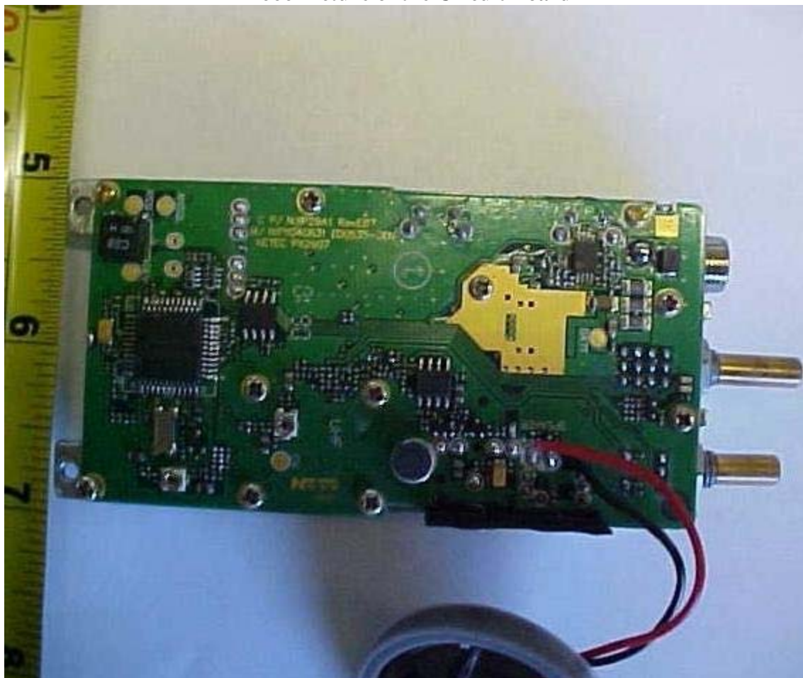
PX - 666 Picture of the Circuit Board #4
