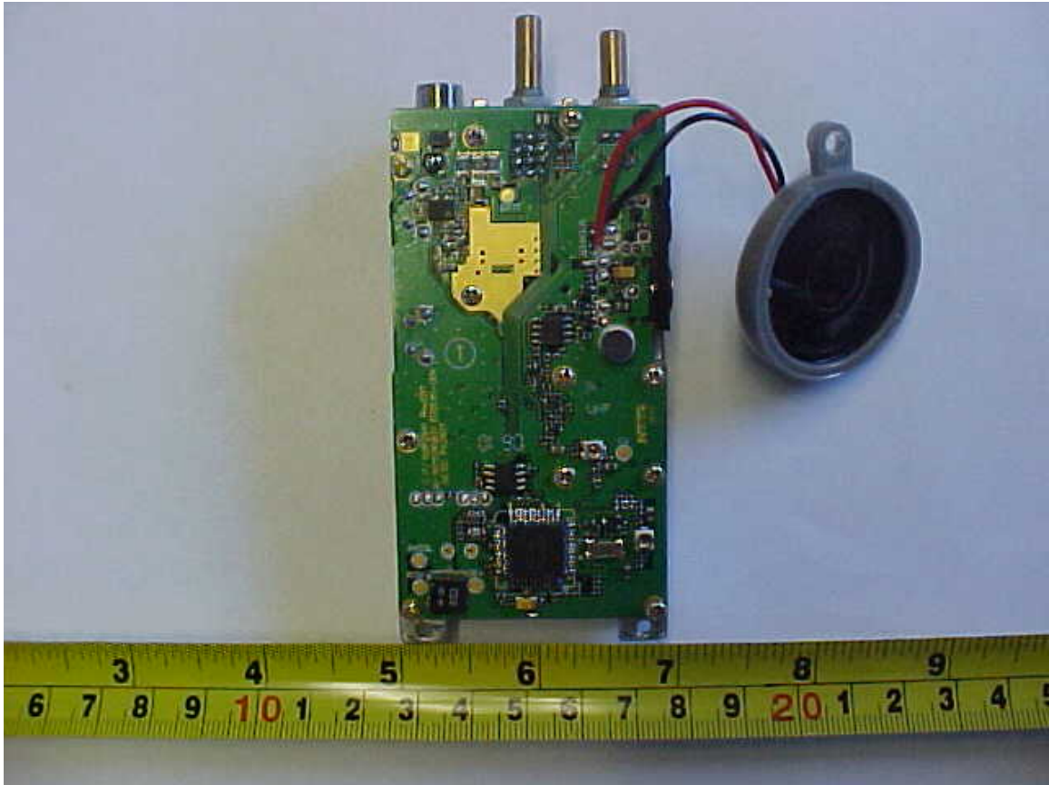
PX - 666 Picture of the Circuit Board #3
