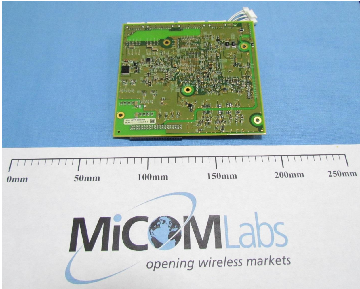
Bottomside - Controller Board P/N: 13029025-320
