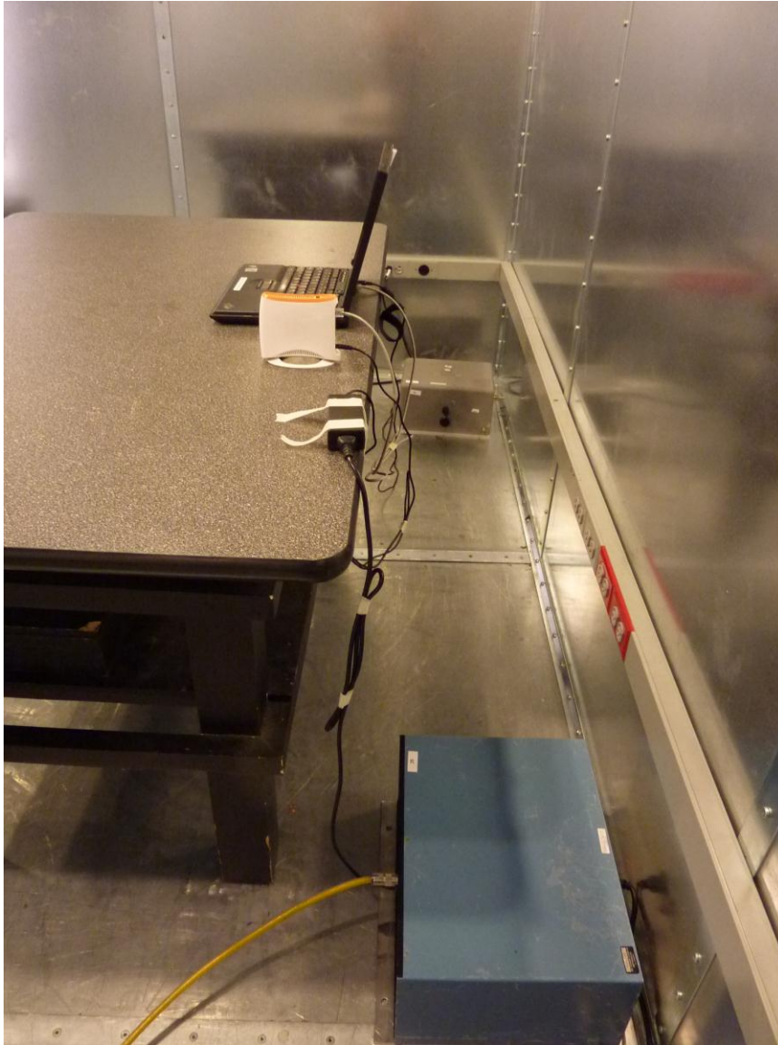
Figure 9: AC Conducted Emission Test Setup for RAP-3WNP (Side View)
