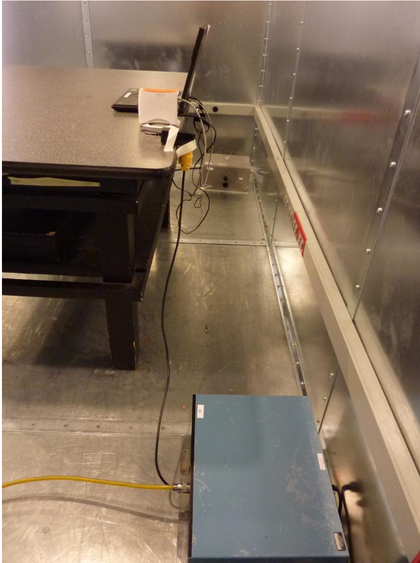
Figure 11: AC Conducted Emission Test Setup for RAP-3WN (Side View)
