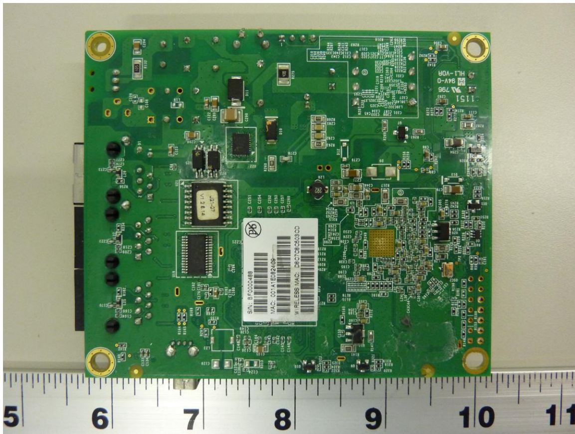
Figure 2: RAP-3WNP – Soldered Side
