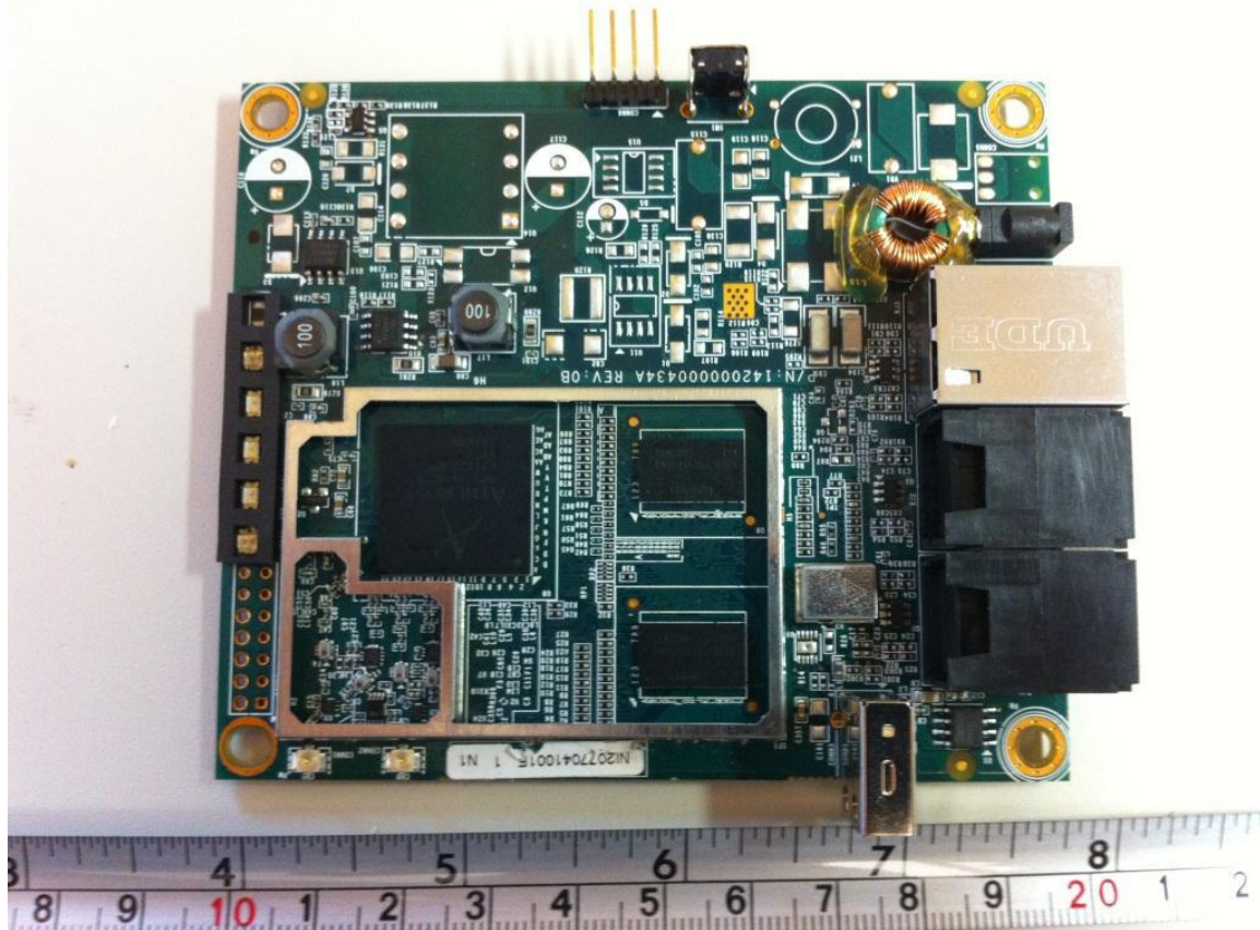
Figure 5: Chipset w/o RF Shielding.
