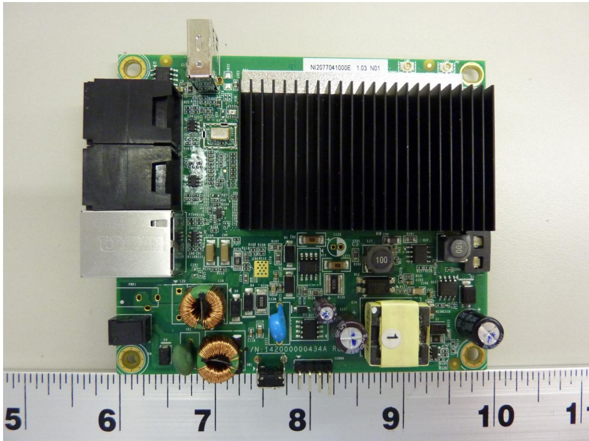
Figure 1: RAP-3WNP – Component Side
