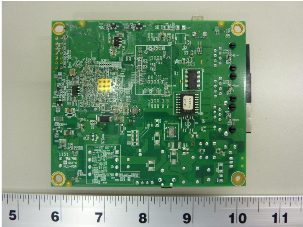
Figure 4: RAP-3WN – Soldered Side
