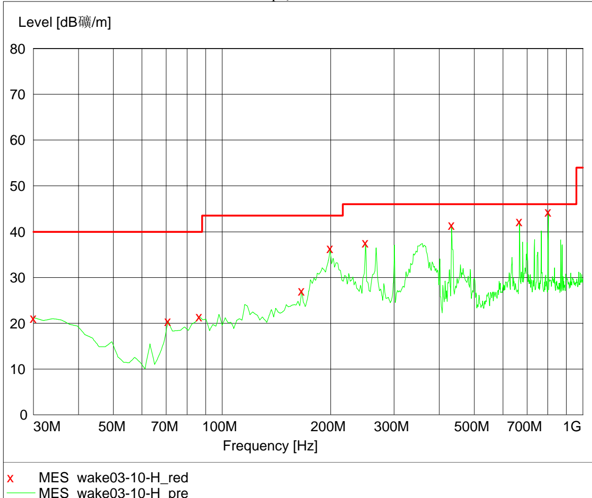
10Mbps, Horizontal
