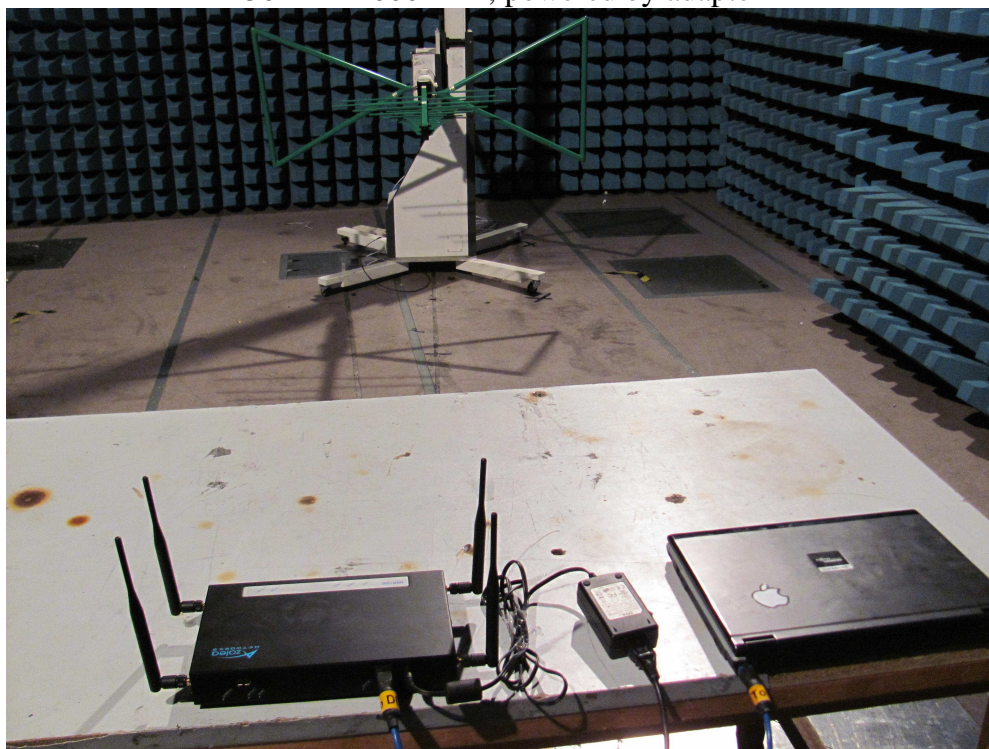
30MHz-1000MHz, powered by adapter
