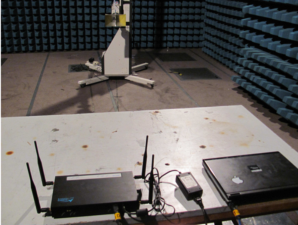
Higher than 1GHz, powered by adapter
