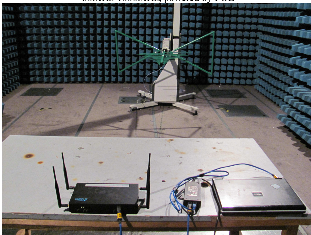
30MHz-1000MHz, powered by POE
