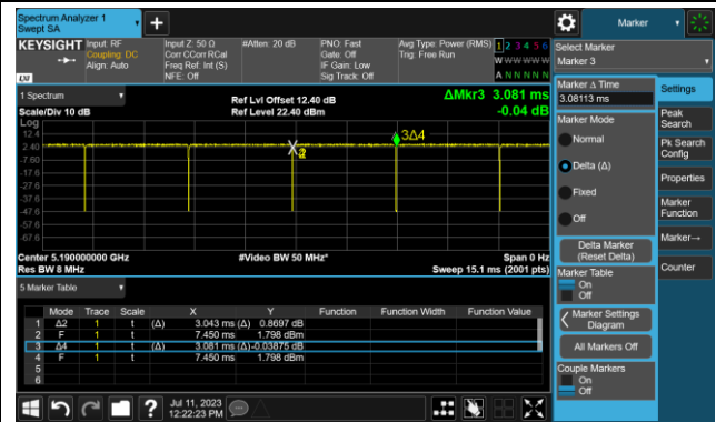
802.11ax-HE40 (T = 3.043ms)
