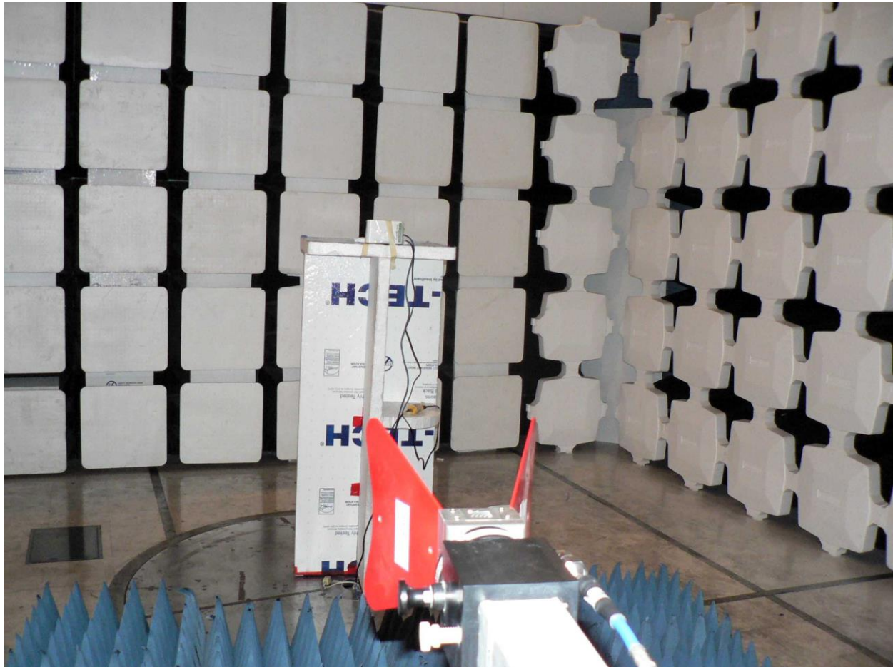
TX Spurious Emissions 1-18GHz Front View
