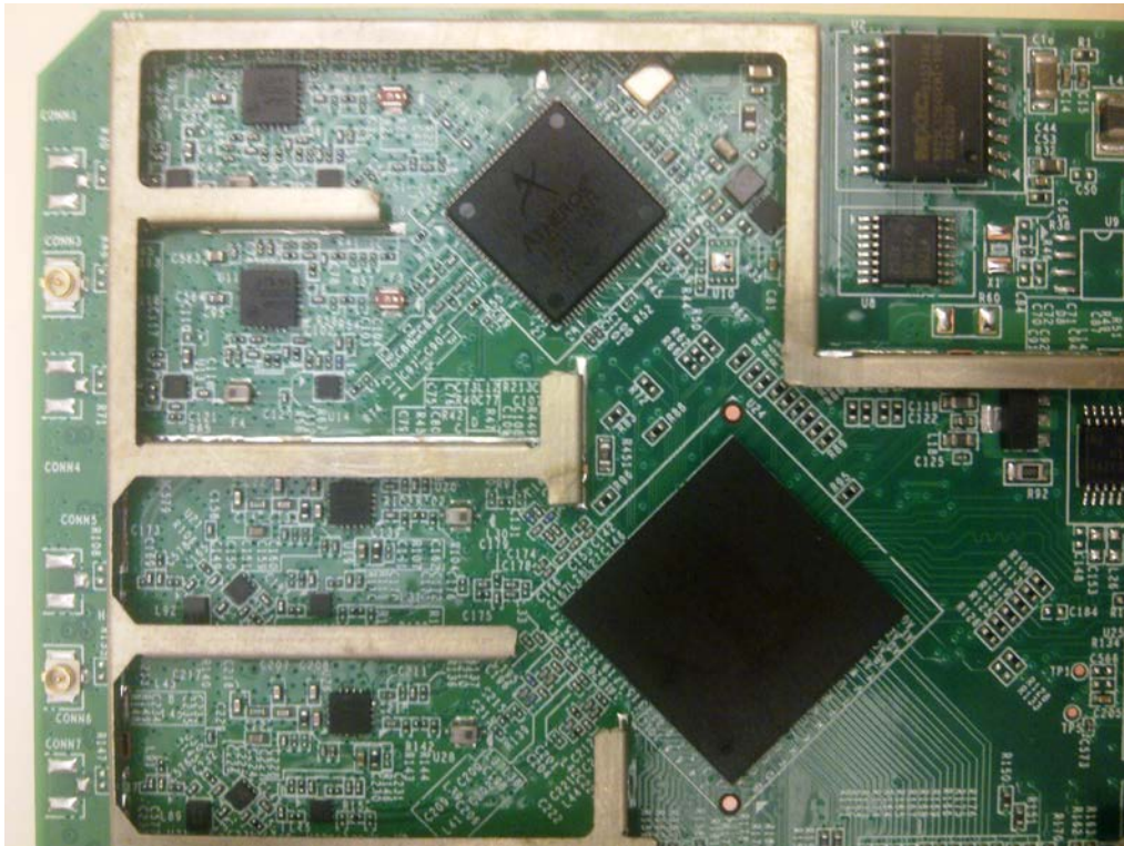
Photo 6 – APINR108 & APINR109 Main Board Radio part shield removed
