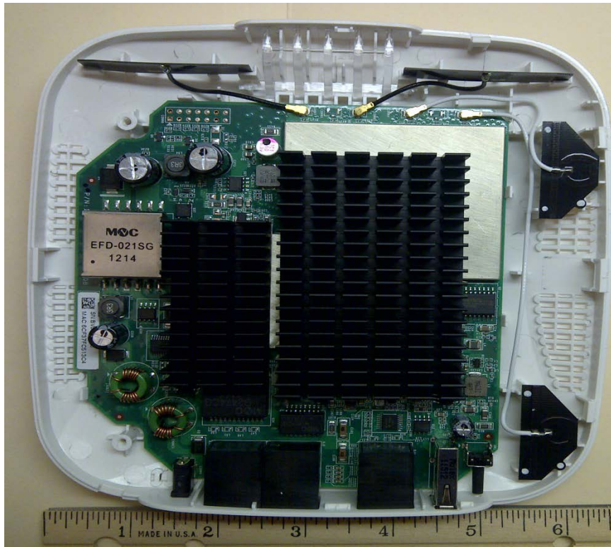
Photo 2 – APINR10p Assembly
