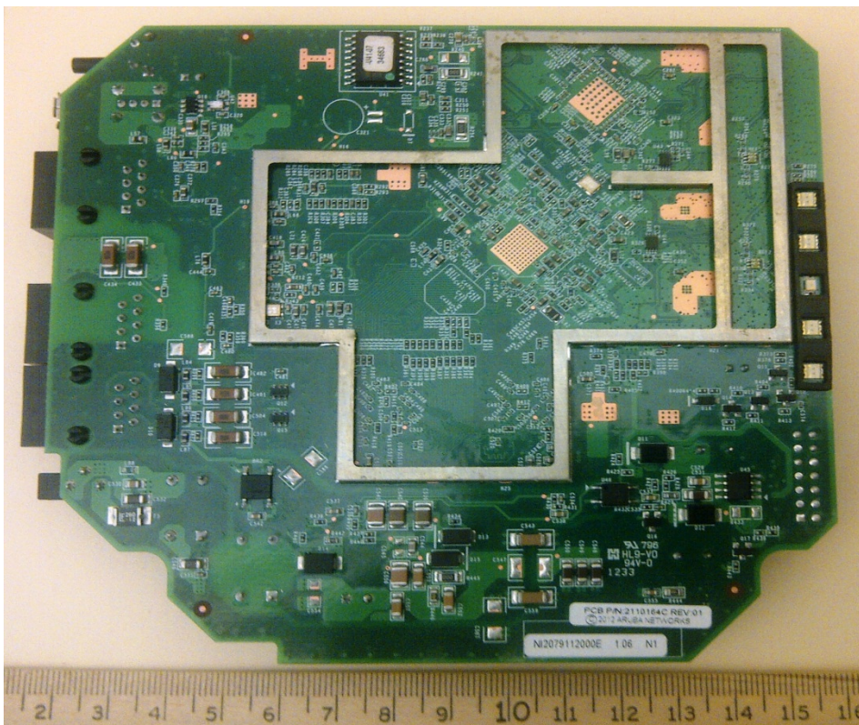
Photo 4 – Main Board Back View shield removed
