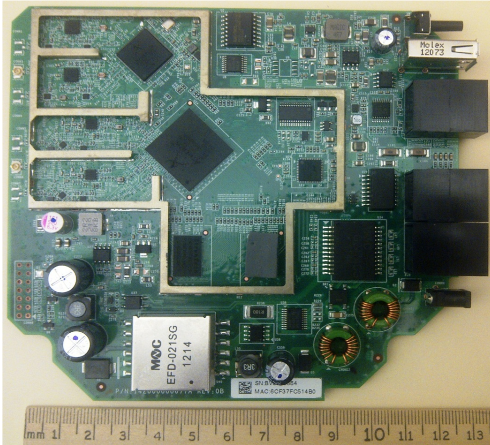
Photo 5 – Main Board Top View shield removed
