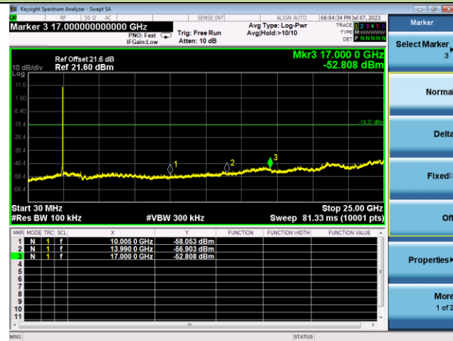
Spurious Emission
