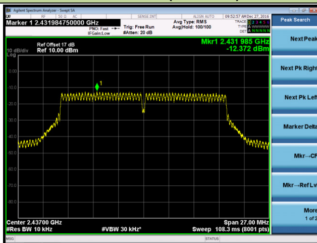
Channel 06 (2437MHz)
