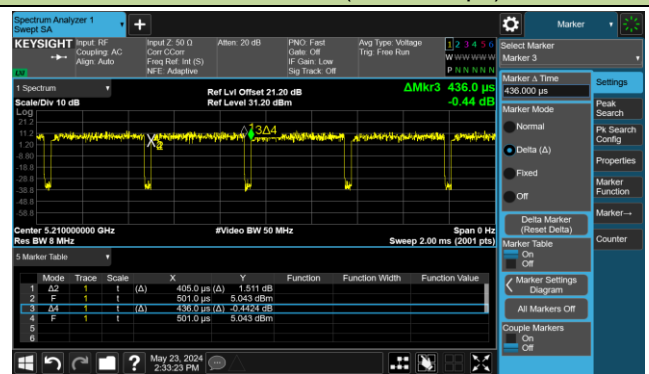
802.11be-EHT20 (T = 1.493ms)
