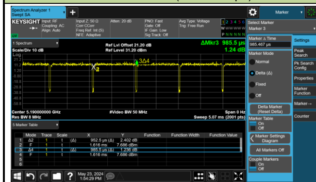
802.11ac-VHT40 (T = 952.5μs)
