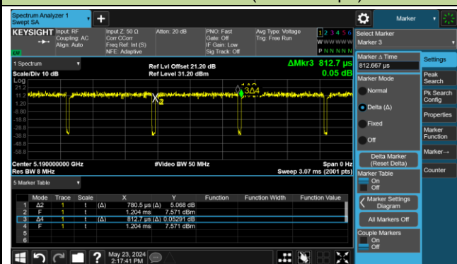
802.11be-EHT40 (T = 780.5µs)
