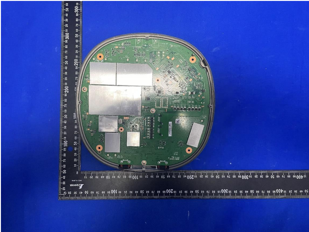
(5) EUT Photo (Model: APIN0735)
