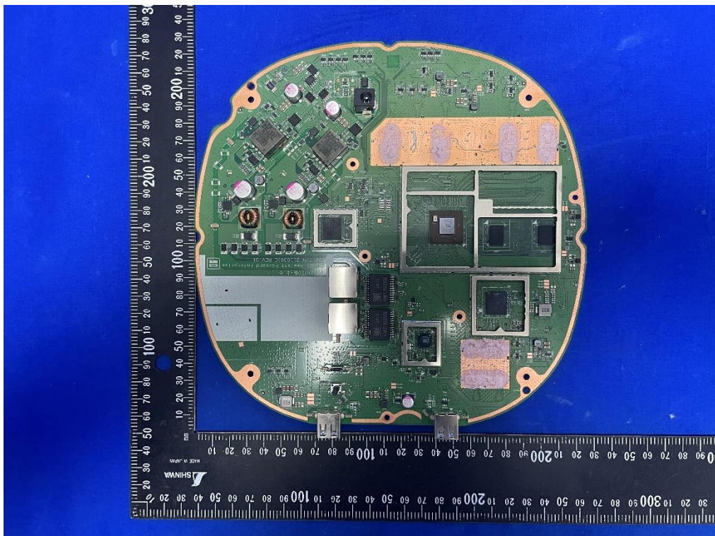
(10) EUT Photo (Model: APIN0735)
