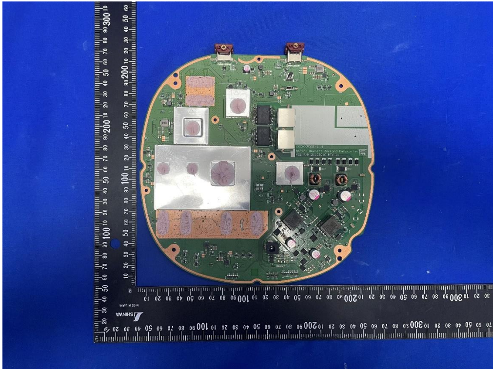
(7) EUT Photo (Model: APIN0735)
