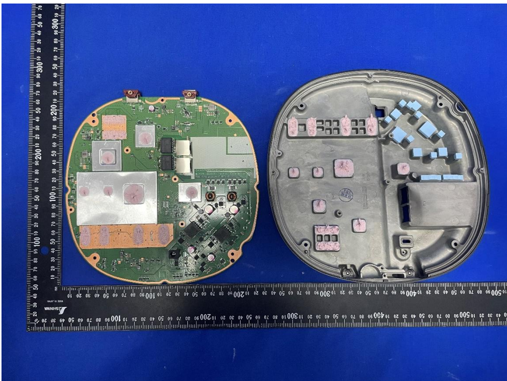
(6) EUT Photo (Model: APIN0735)
