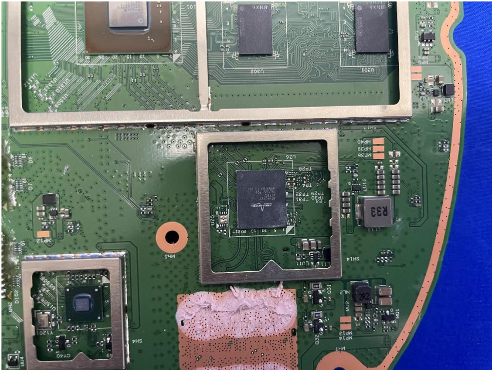
(12) EUT Photo (Model: APIN0735)
