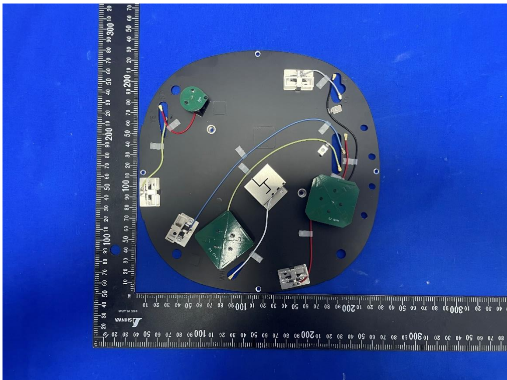
(4) EUT Photo (Model: APIN0735)
