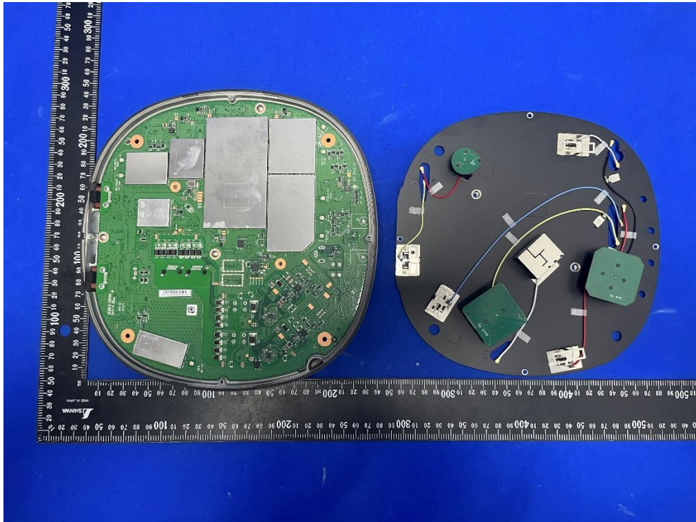
(3) EUT Photo (Model: APIN0735)
