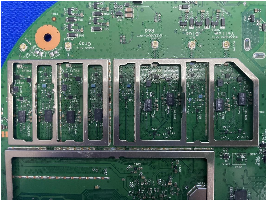
(17) EUT Photo (Model: APIN0735)
