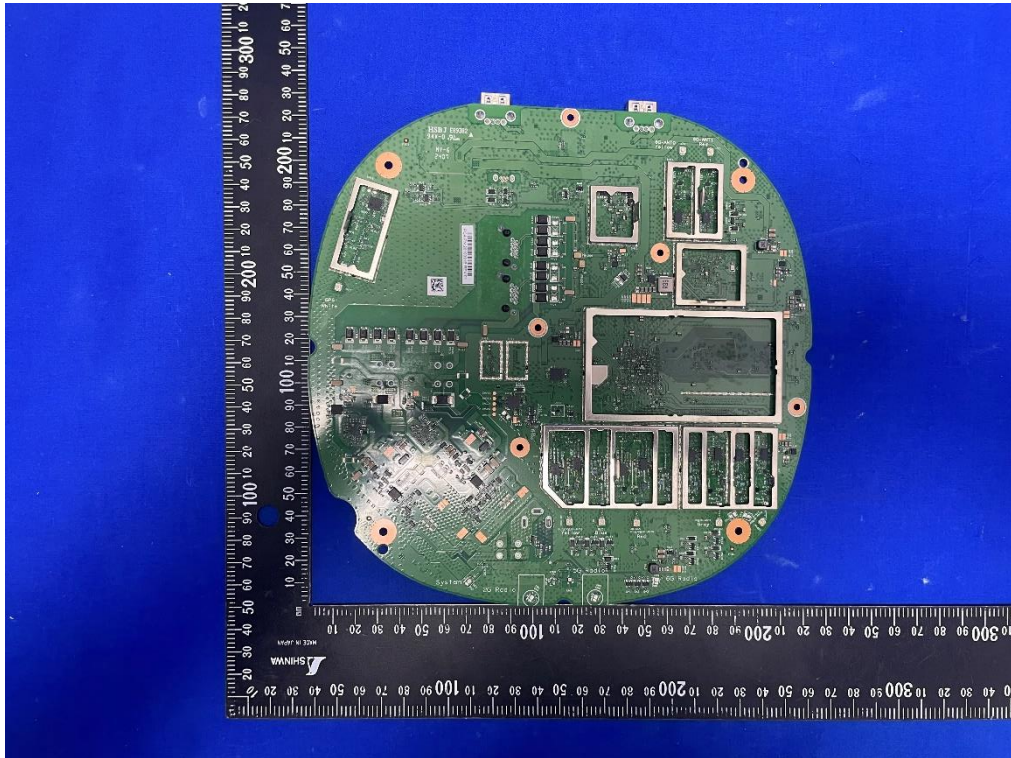
(9) EUT Photo (Model: APIN0735)
