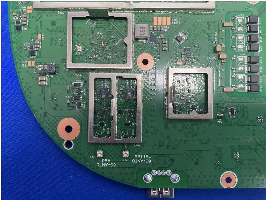
(15) EUT Photo (Model: APIN0735)
