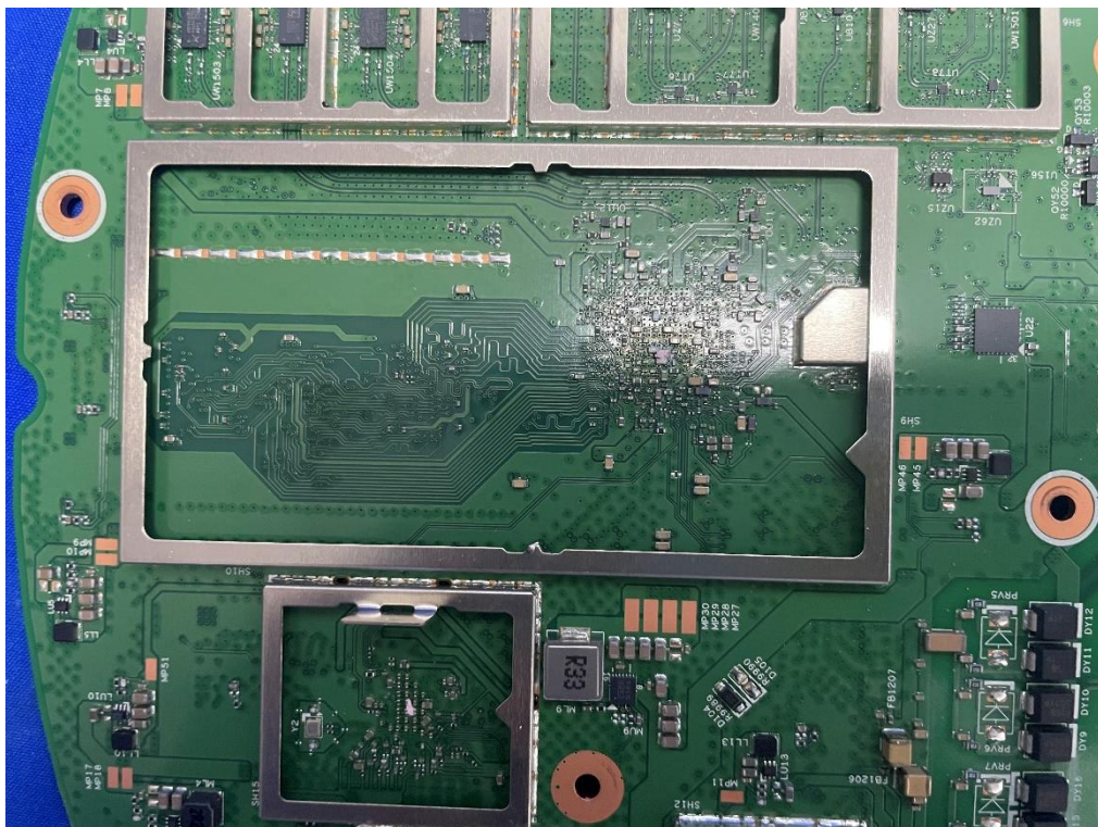
(16) EUT Photo (Model: APIN0735)
