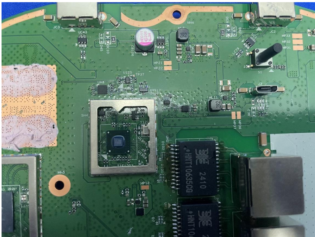
(14) EUT Photo (Model: APIN0735)
