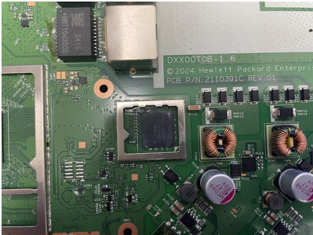
(13) EUT Photo (Model: APIN0735)
