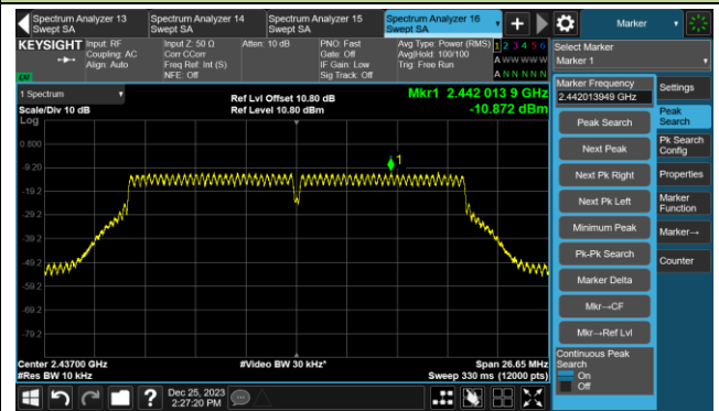
Channel 06 (2437MHz)
