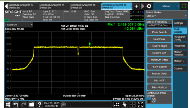
Channel 06 (2437MHz)
