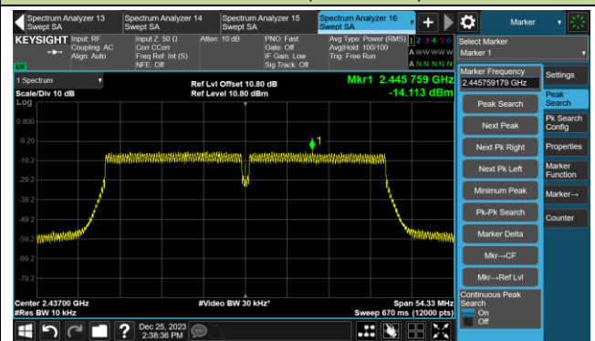
Channel 06 (2437MHz)
