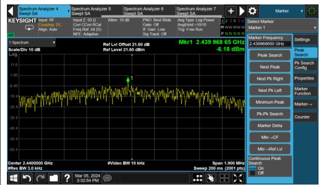
Channel 19 (2440MHz)
