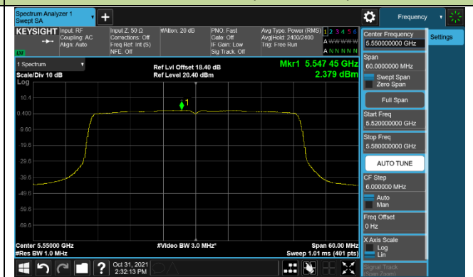
Channel 110 (5550MHz)
