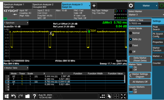
802.11ax-HE80+80 (T = 5.444ms)
