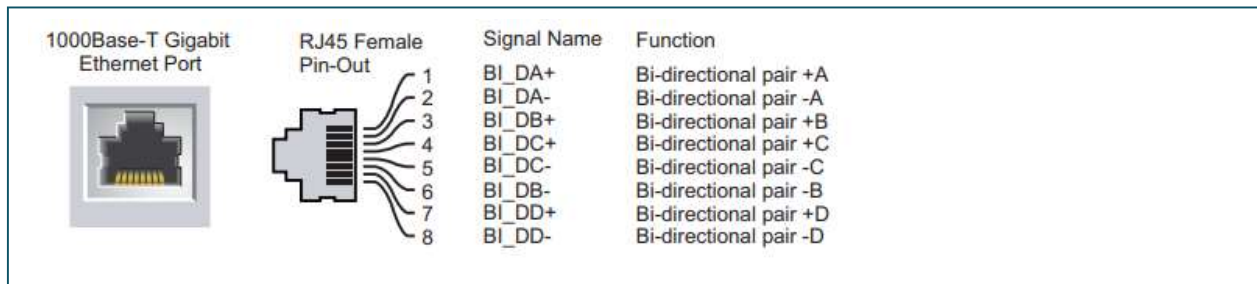
Figure 10 100/1000/2500/5000 Base-T
