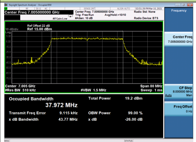
Channel 211 (7005MHz)
