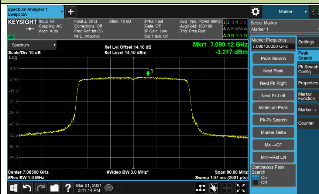
Channel 227 (7085MHz)
