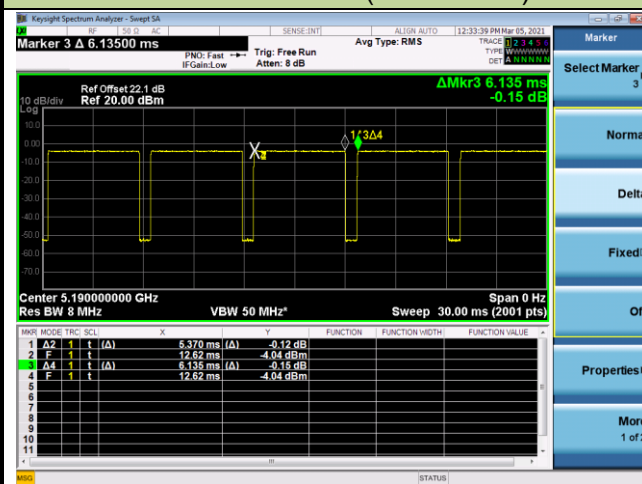
802.11ac-VHT40 (T=5.370ms)
