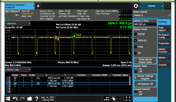
802.11ac-VHT80 (T=0.456ms)
