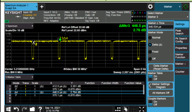
802.11ax-HE80 (T=0.413ms)
