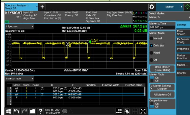
802.11ax-HE160 (T=0.235ms)
