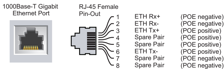
Figure 6 Ethernet Port Pin-Out
