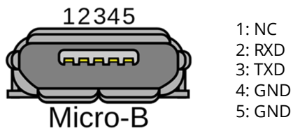
Figure 5 Micro-B Port Pin-out
