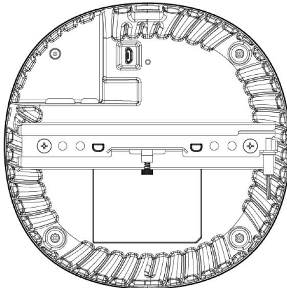
Figure 4 Access Point Rear View
