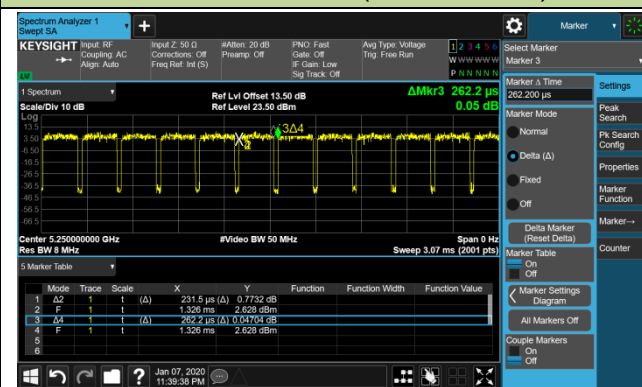
802.11ax-HE160 (T = 231.5us)
