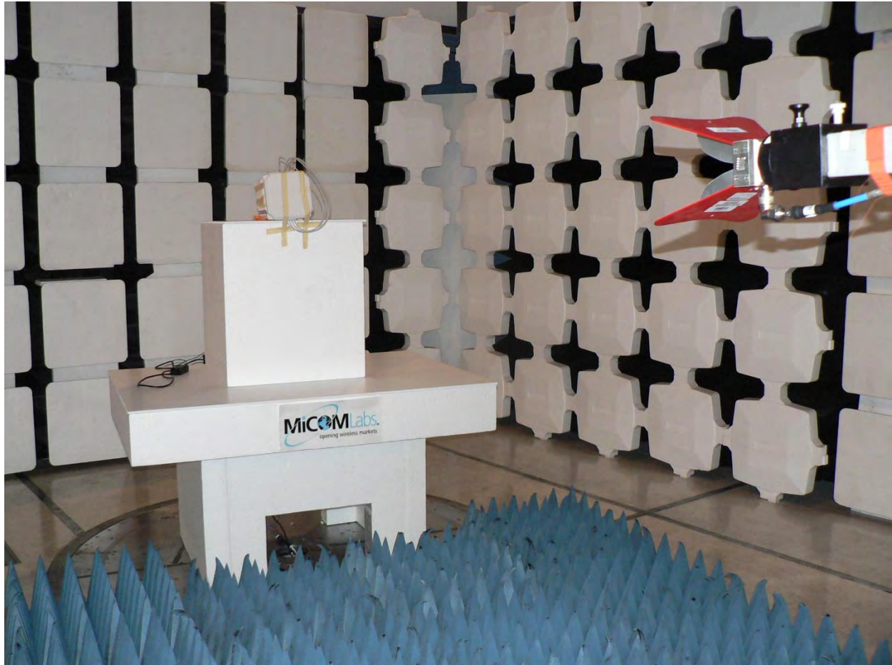
HPEN111 AP344 AP- ANT-45 Transmitter Spurious
