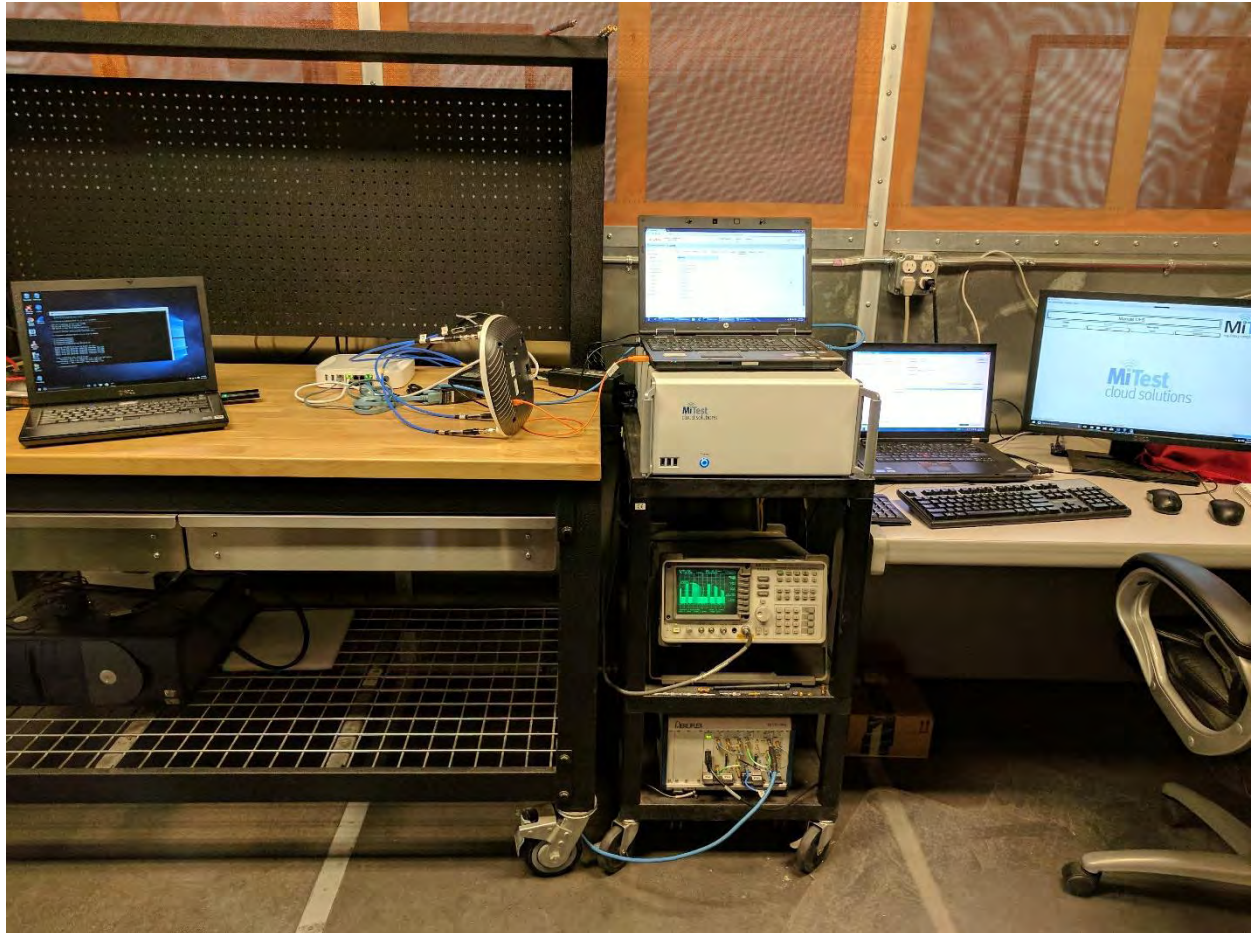
HPEN111 AP344 Conducted DFS Setup
