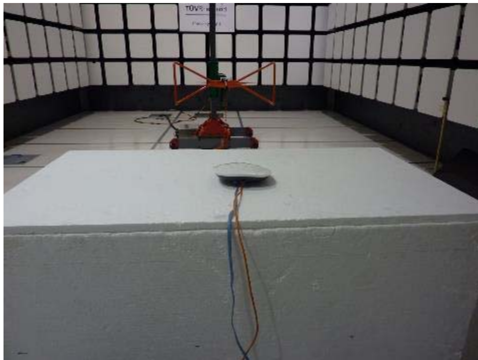
30MHz to 1000MHz APIN0325
