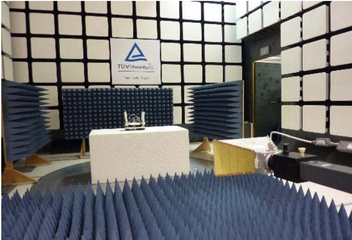
1 to 18GHz APIN0324 with AP-ANT-19
