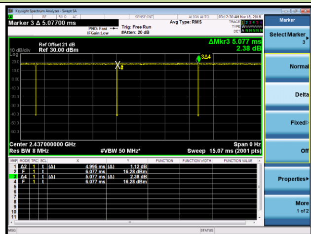
802.11n-HT20 (T = 4.995ms)
