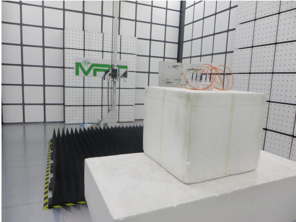
Description: Radiated Spurious Emission Test Setup for 18GHz ~ 40GHz (Directional Antenna: ANT-2x2-2314 & ANT-4x4-5314)
