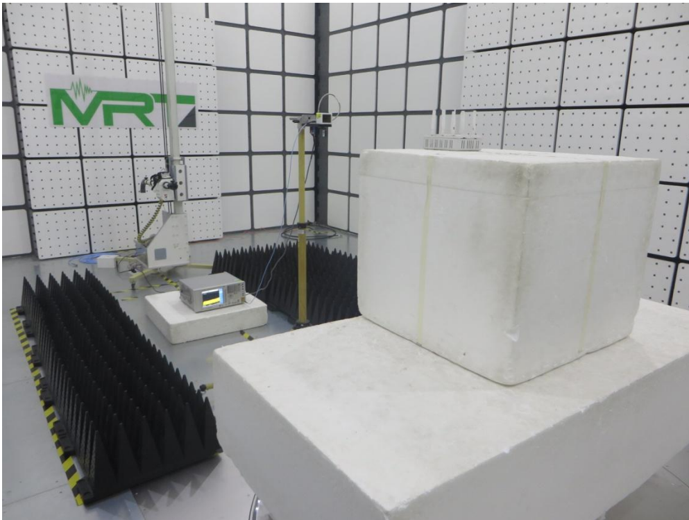
Description: Radiated Spurious Emission Test Setup for 18GHz ~ 40GHz (Omni Antenna: AP-ANT-20W)
