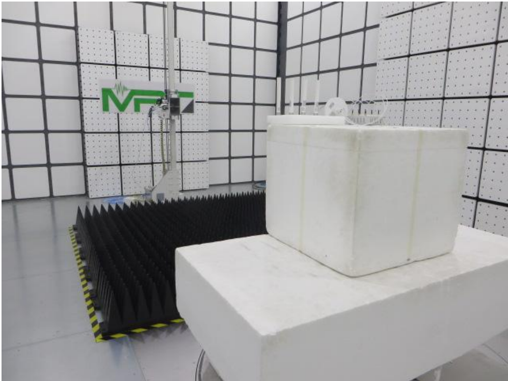
Description: Radiated Spurious Emission Test Setup for 18GHz ~ 40GHz (AP-ANT-19 + AP-ANT-40)
