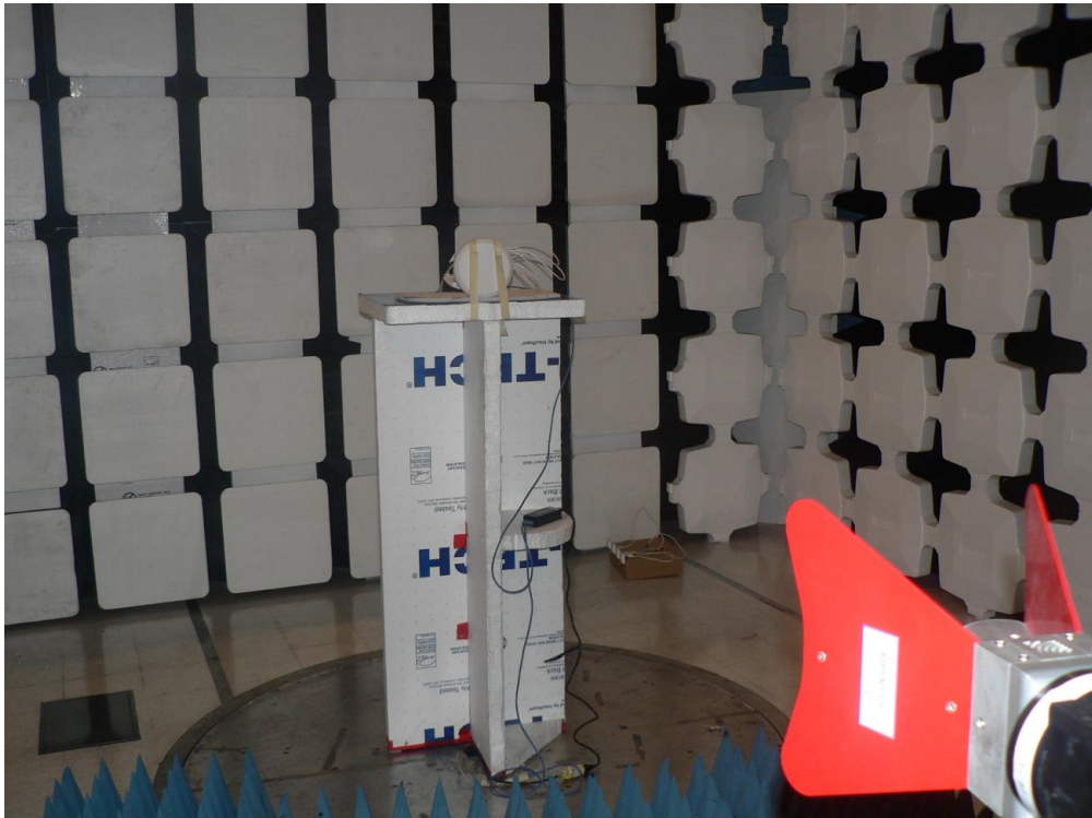
ANT45- Antenna 1-18 GHz
