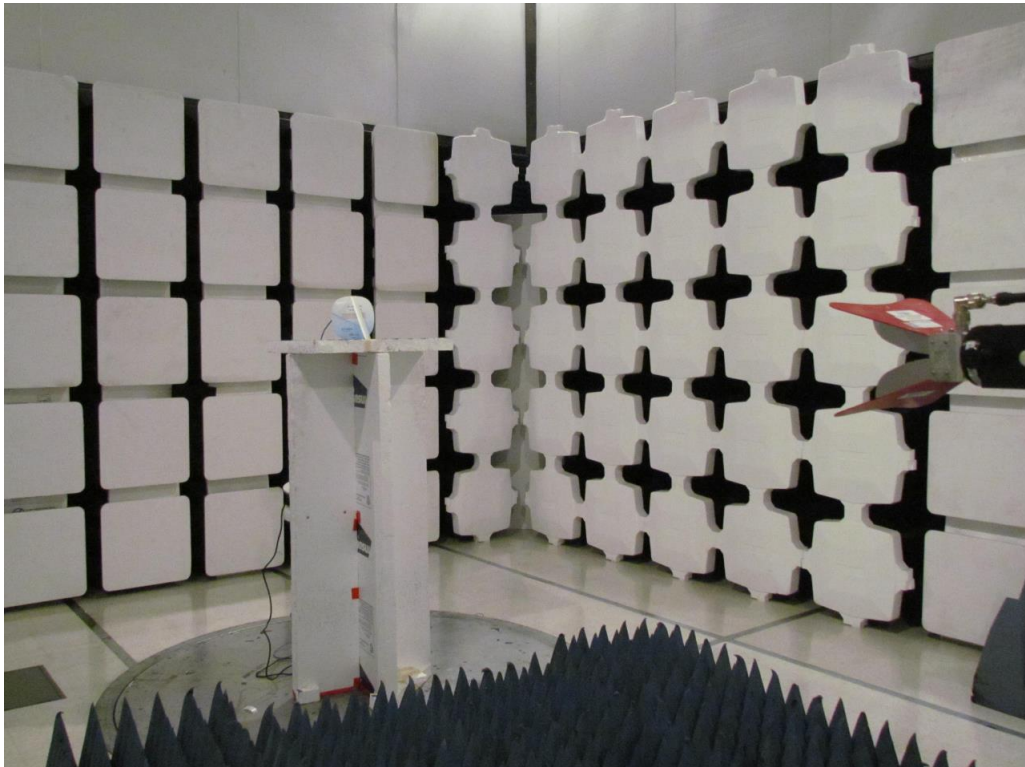
Integral Antenna 1-18 GHz
