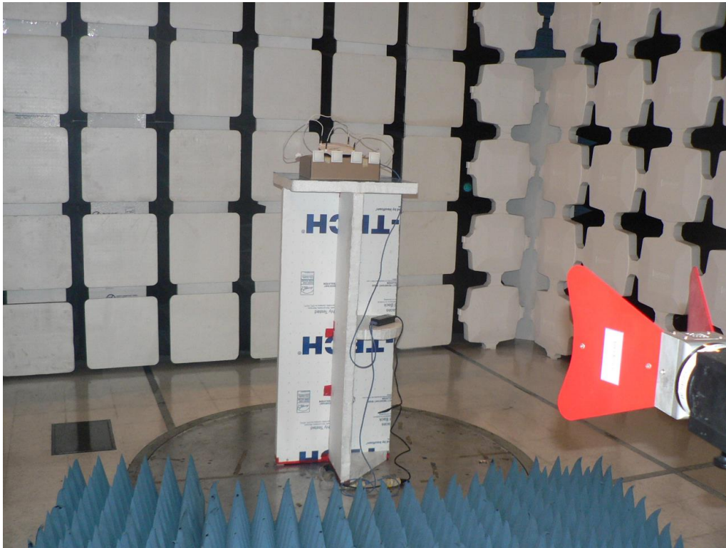
ANT-19 Antenna 1-18 GHz
