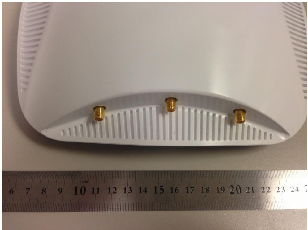
Photo 3 – Ports View
