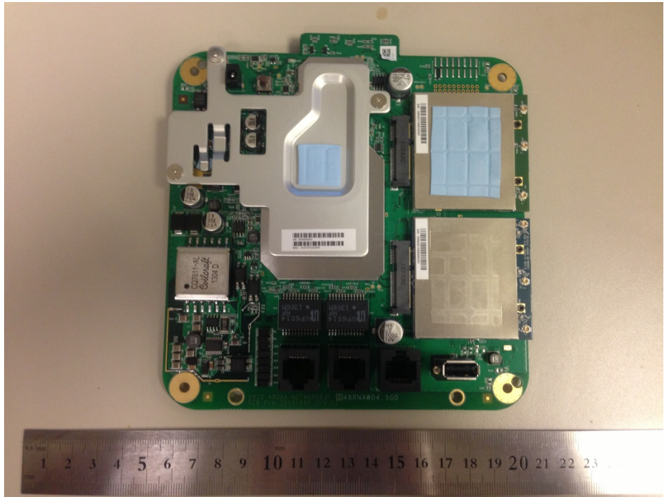
Photo 3 – Main Board Front View
