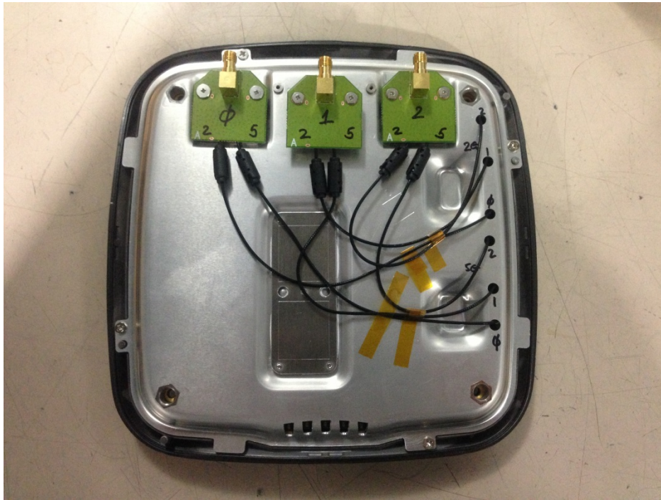
Photo 1 – Cover Shielding view
