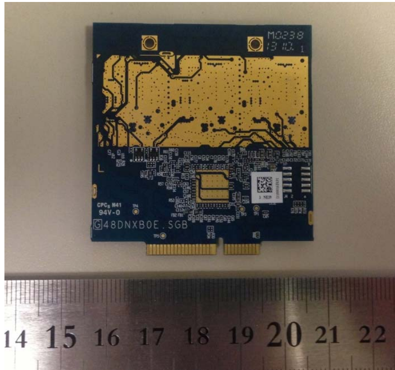
Photo 7- RF module back view
