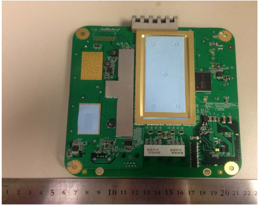
Photo 5 - Main Board Back View
