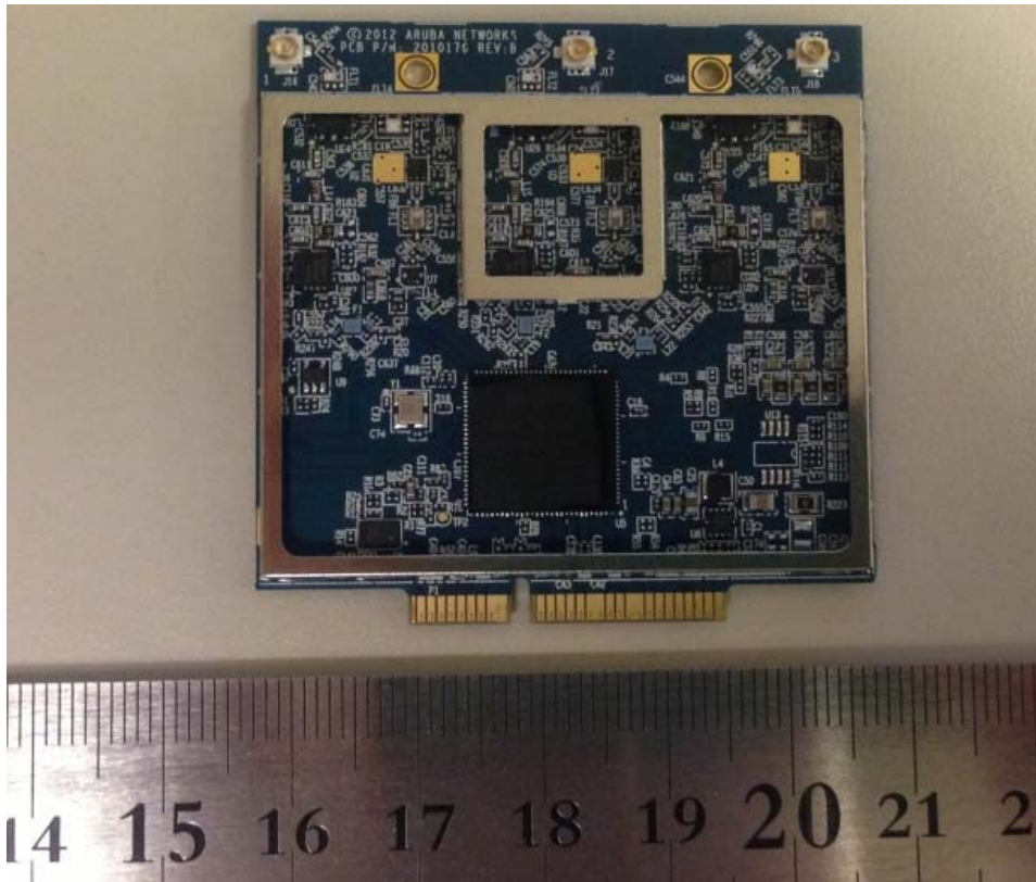
Photo 6- RF module front view(shielding off)
