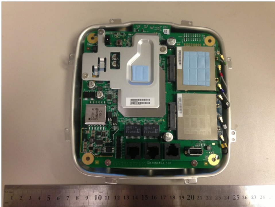
Photo 2 – Cover off Shielding view
