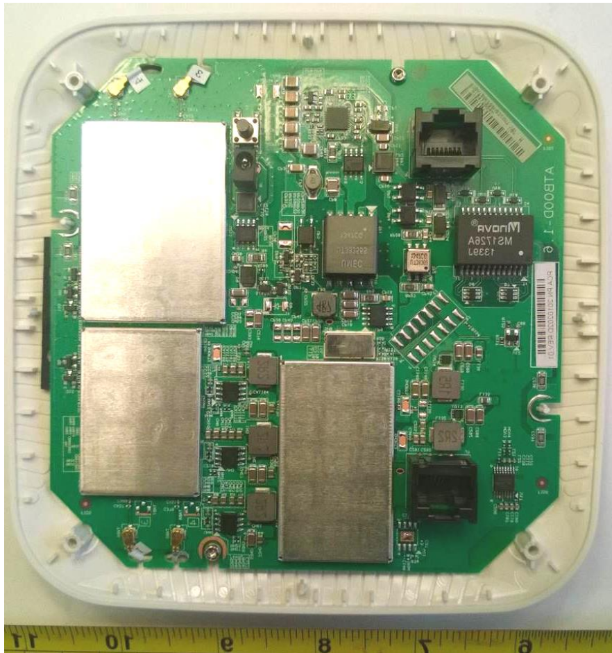
TOP SIDE OF PCB WITH SHIELDS
