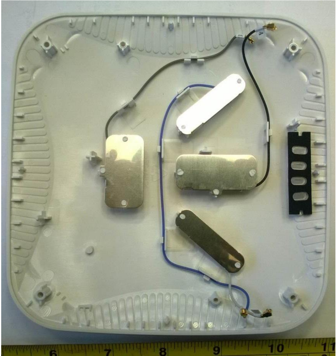
INSIDE OF TOP COVER SHOWING INTERNAL ANTENNAS
