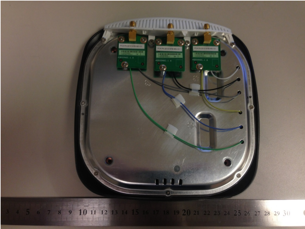
Photo 1 – Cover off shielding view
