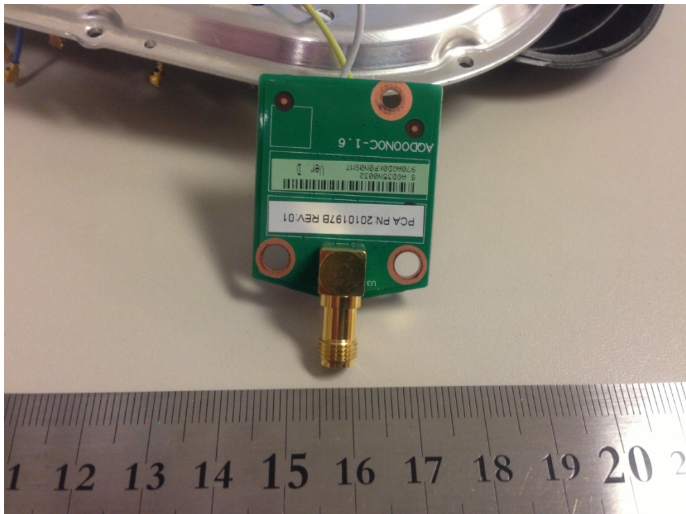
Photo 6- antenna connector front view
