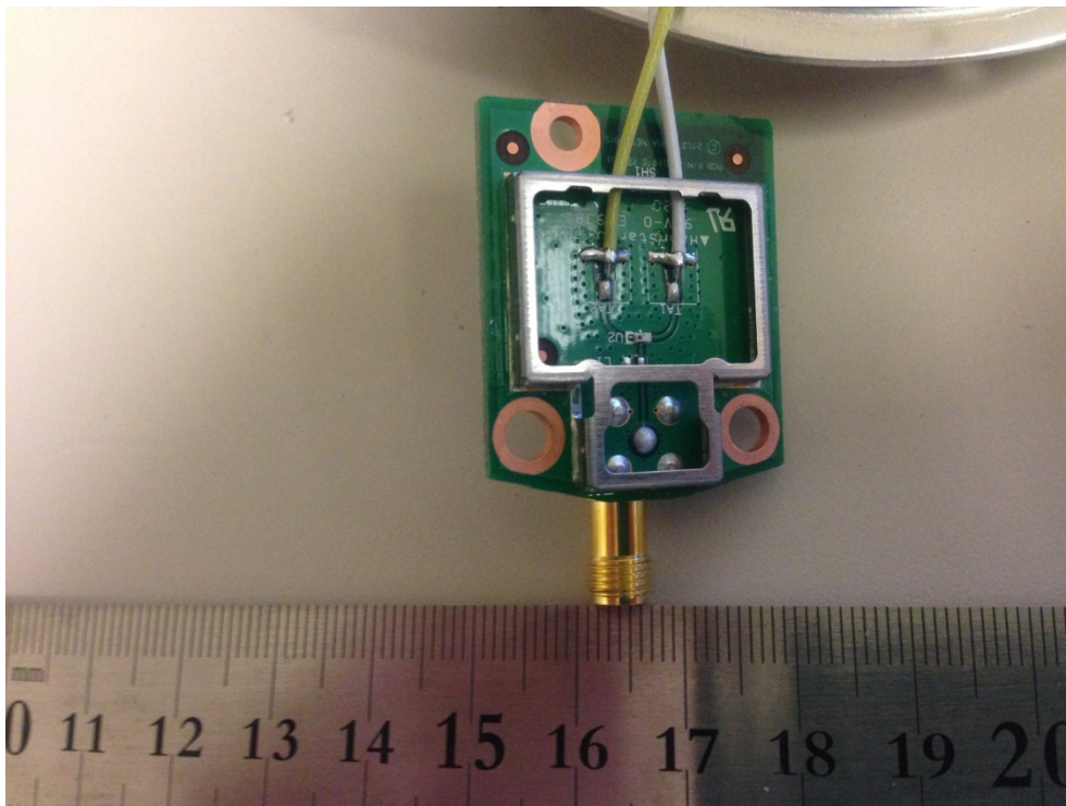
Photo 8- antenna connector back view( shielding off)
