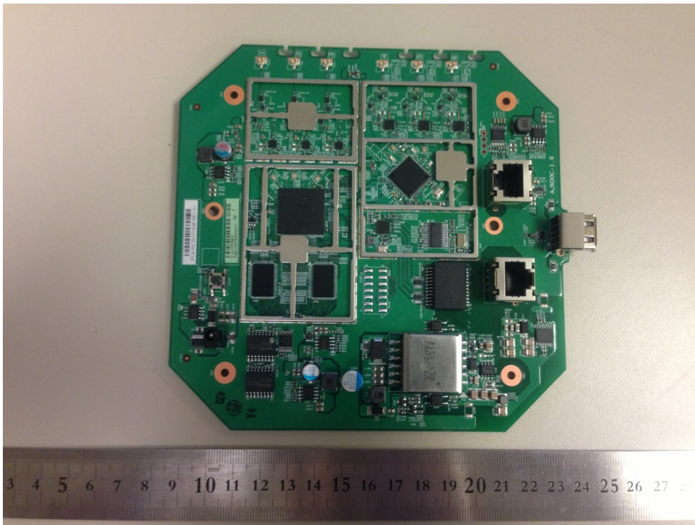
Photo 3- Main Board front View (Shielding off)
