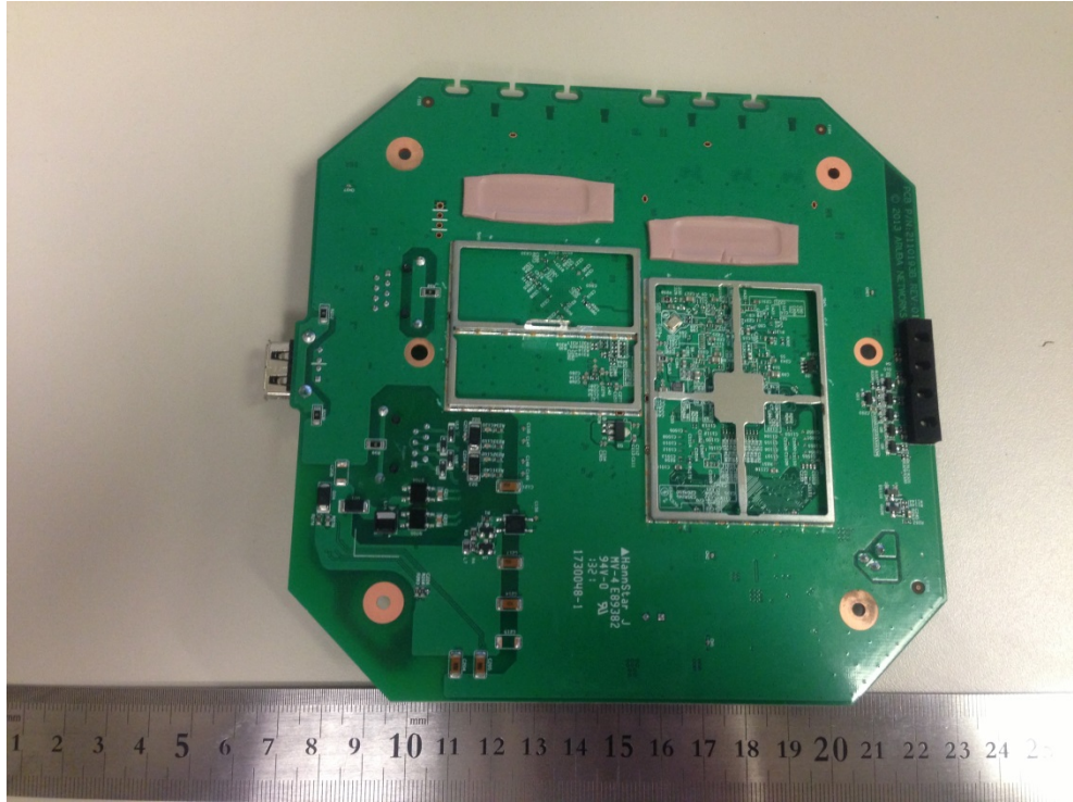
Photo 5- Main Board back View (Shielding off)
