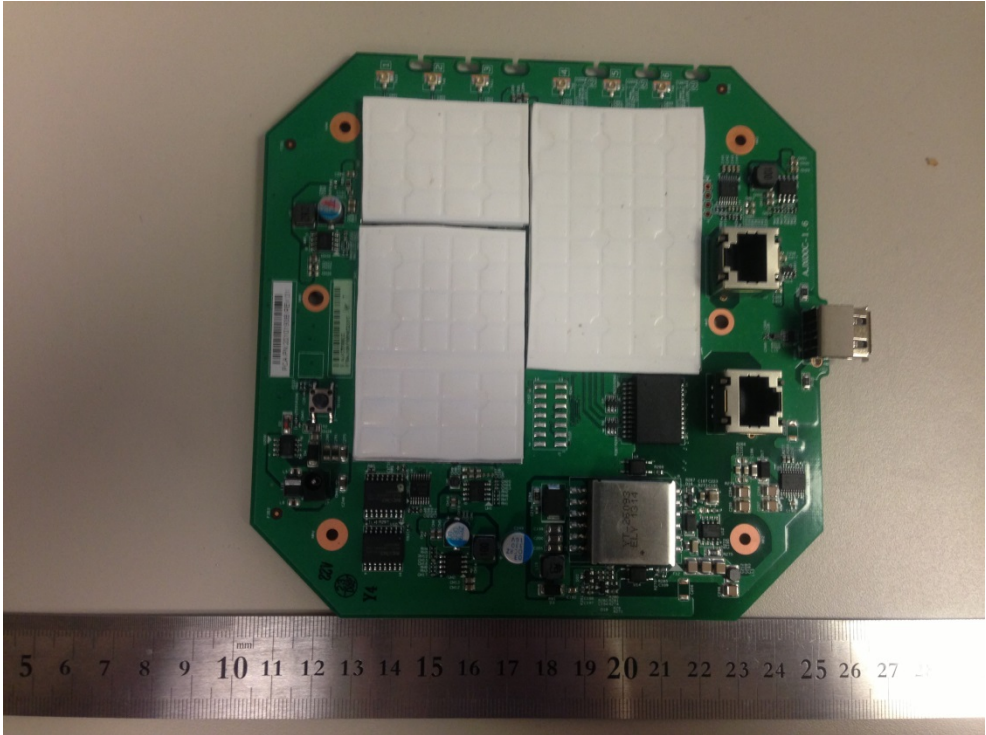
Photo 2 – Main Board Front View
