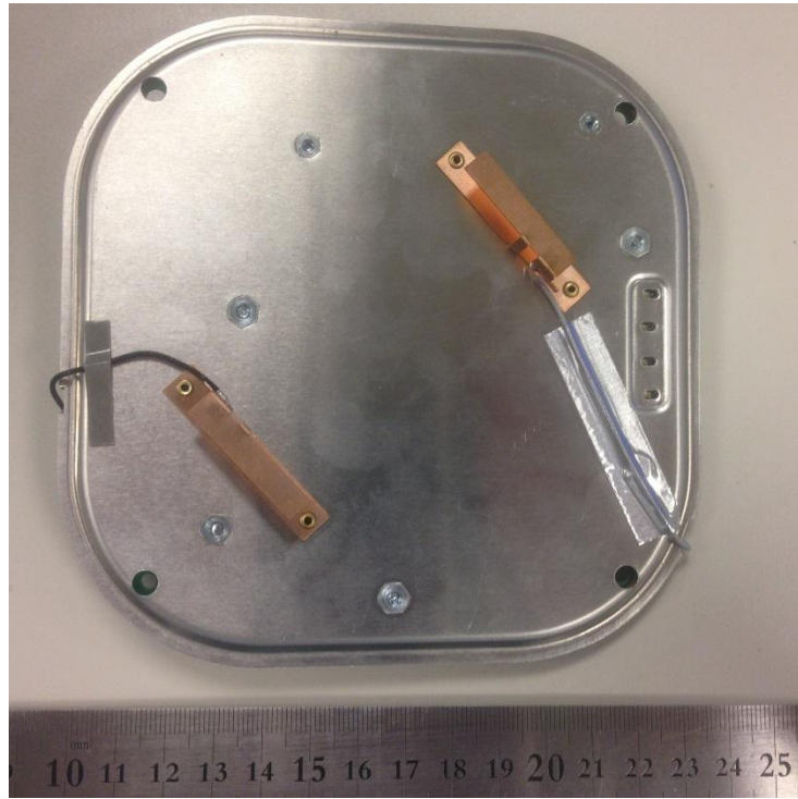
Photo 5 – Main Board Bottom View
