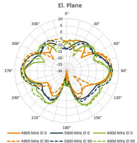
5GHz Wi-Fi band antenna patterns (vertical)
