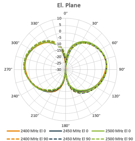
2.4GHz Wi-Fi band antennas patterns (vertical)
