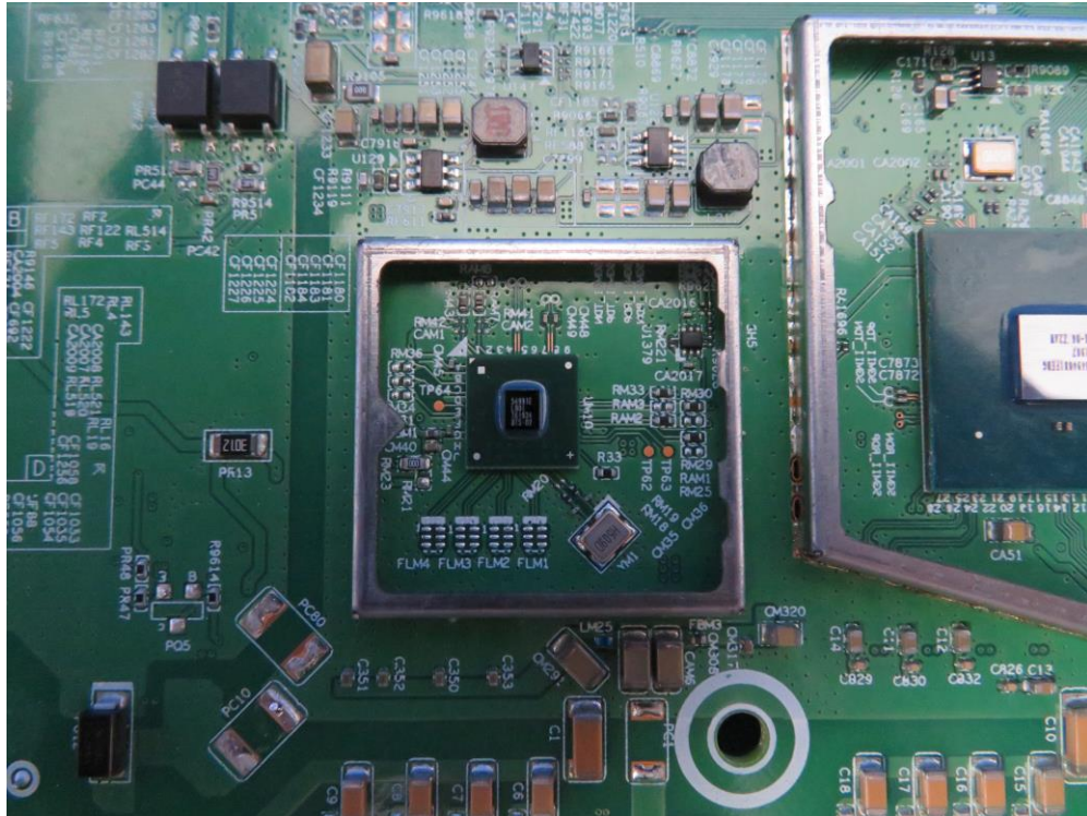
(27) EUT Photo (For all models)
