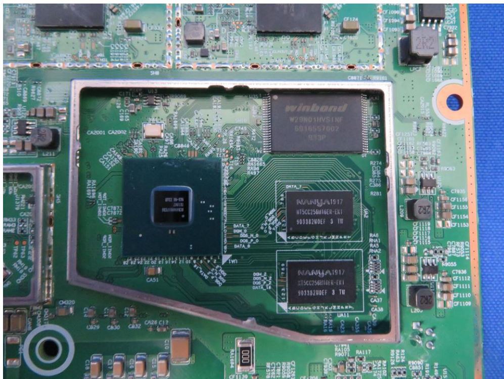
(26) EUT Photo (For all models)
