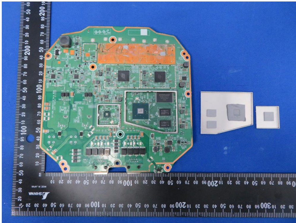
(25) EUT Photo (For all models)
