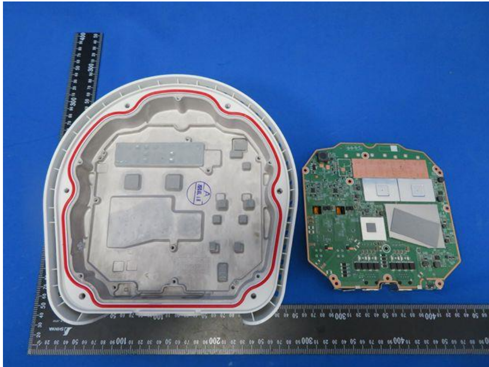
(15) EUT Photo (APEX0577)
