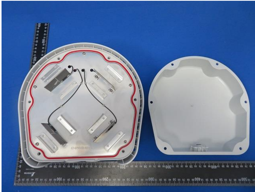
(11) EUT Photo (APEX0577)
