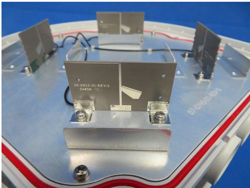
(12) EUT Photo (APEX0577)
