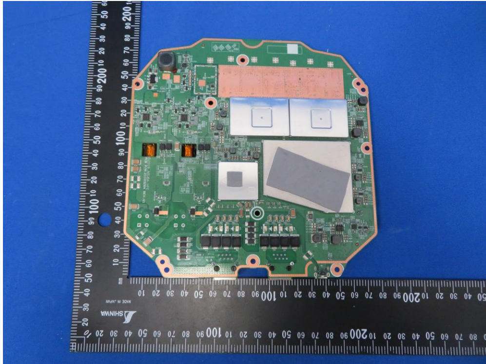
(17) EUT Photo (APEX0577)
