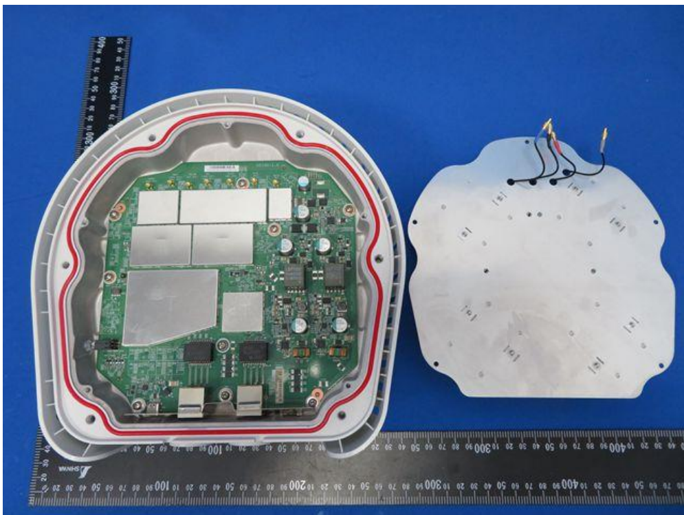
(14) EUT Photo (APEX0577)
