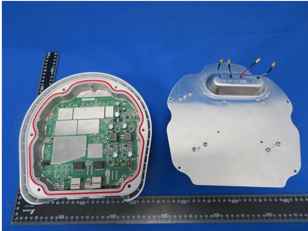
(7) EUT Photo (APEX0575)
