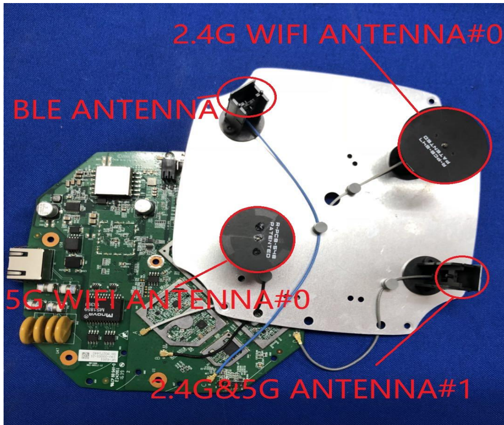
(7) EUT Photo ( APEX0365 )
