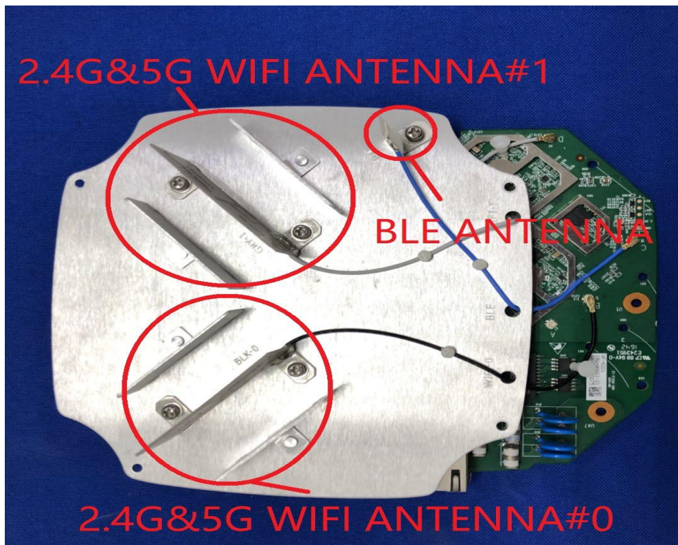
(14) EUT Photo ( APEX0367 )
