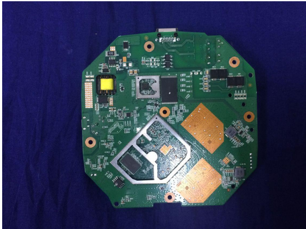
(8) EUT Photo ( APEX0367 )
