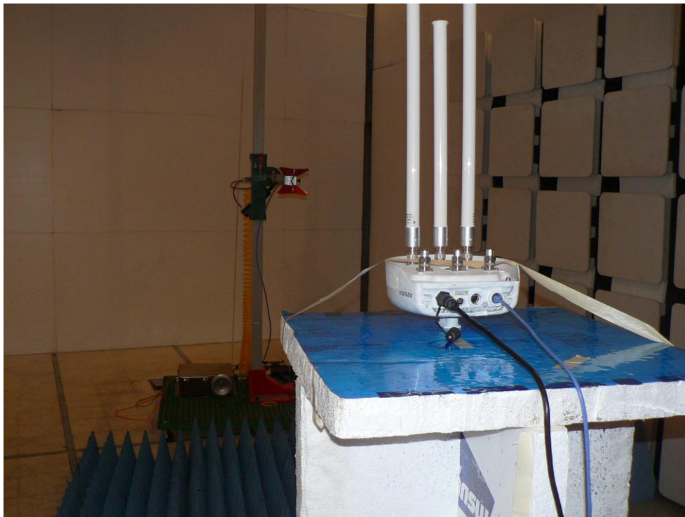
AP274 ANT 5010 TX Spurious Emissions Back
