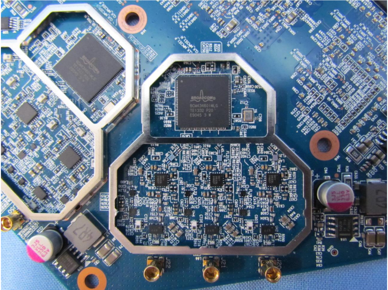
RF Card 2
