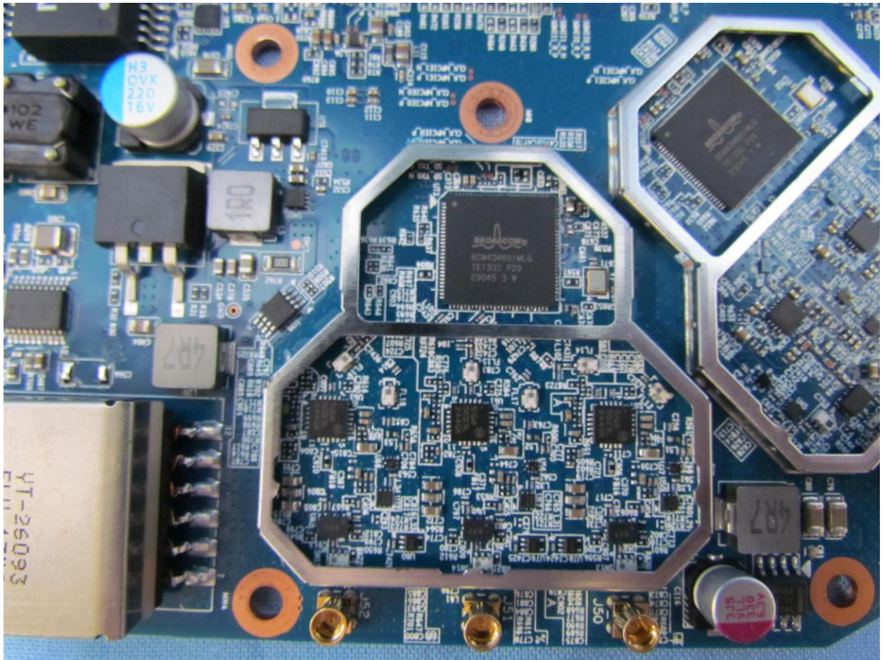
RF Card 1
