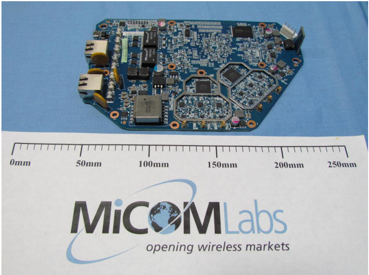
Circuit Board with Shields Off
