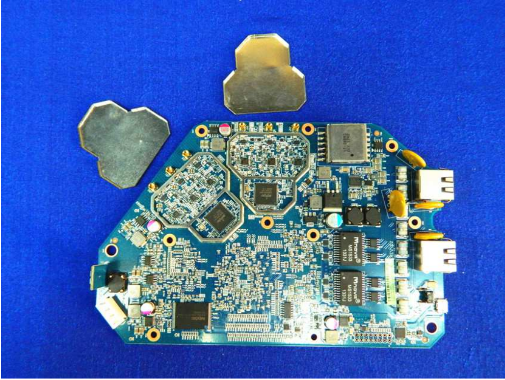
Internal View 5 of PCB
