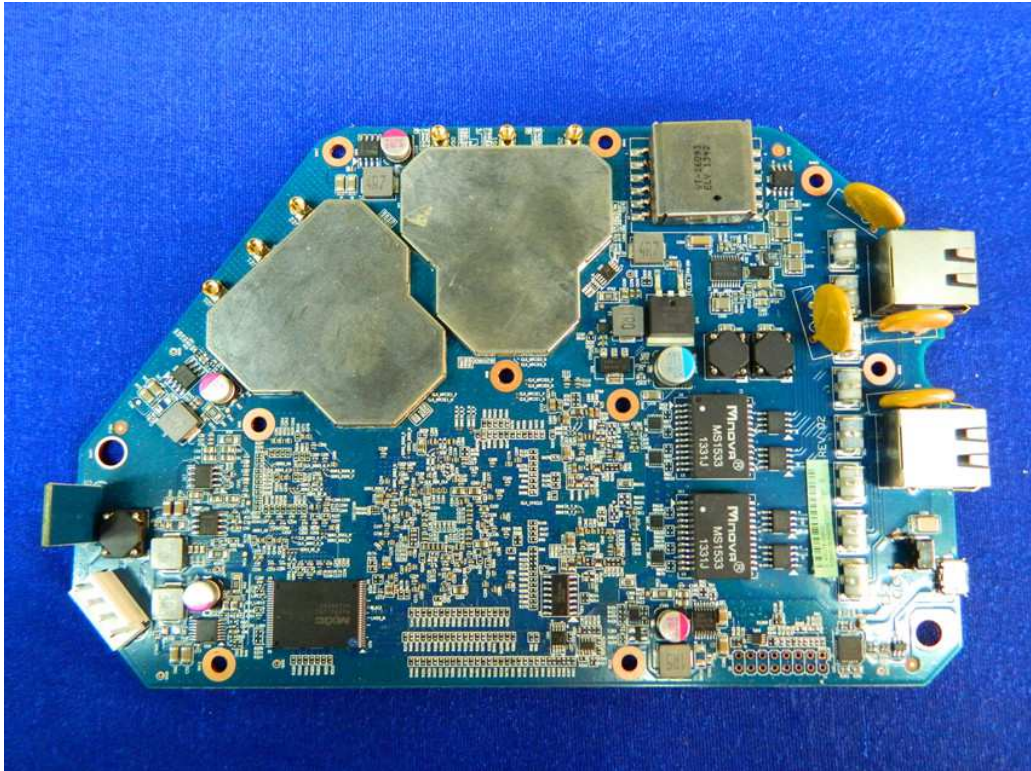
Internal View 3 of PCB
