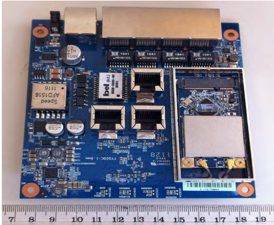
Photo 3 – Main Board Top View (Shielding off)
