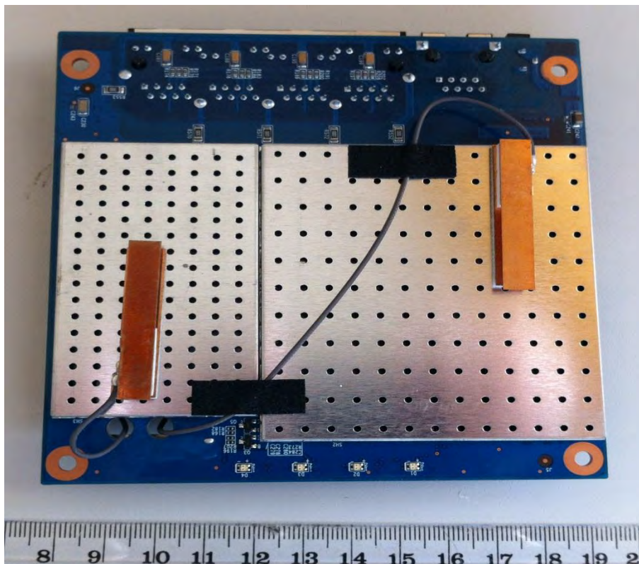
Photo 3 – Main Board Top View (Shielding off)
