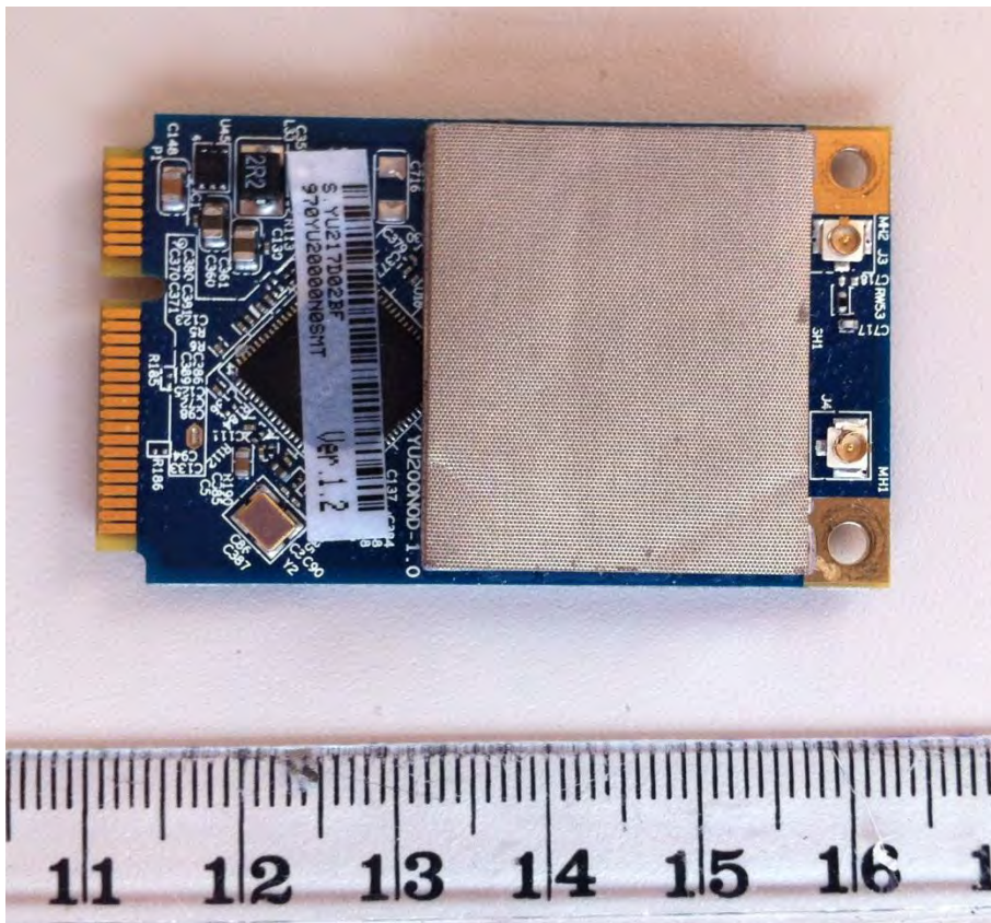
Photo 6 – Radio Card Top View
