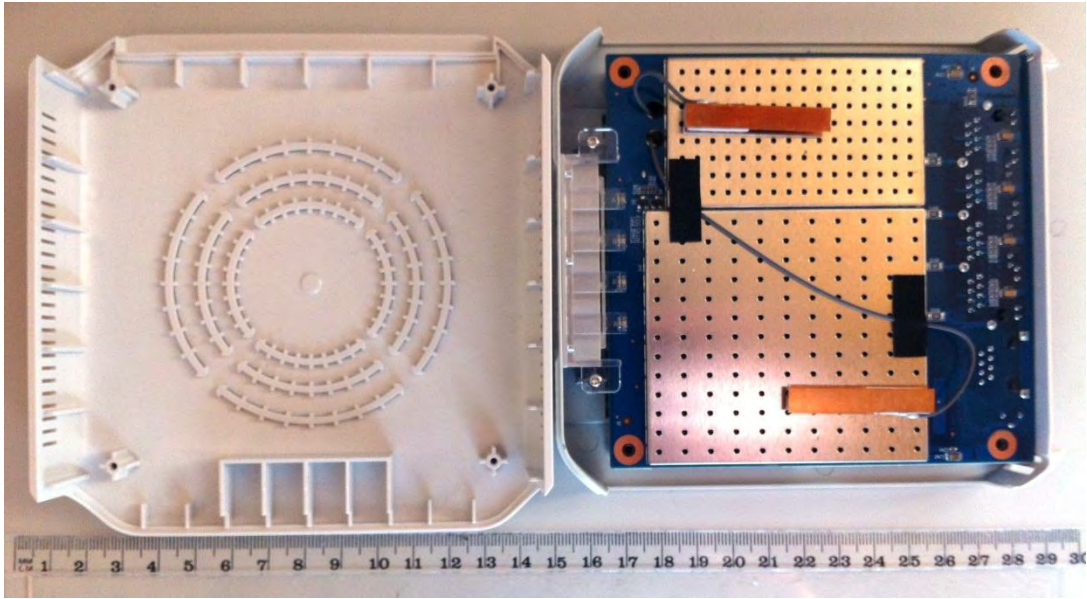
Photo 1 – Cover off View
