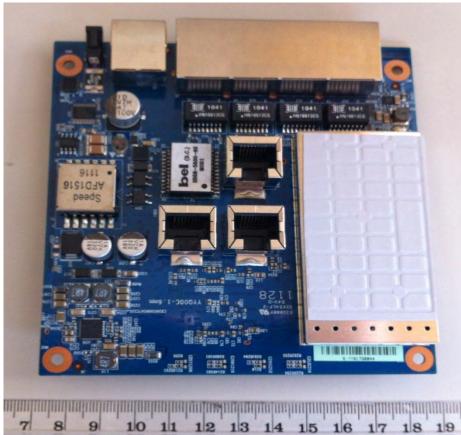
Photo 2 – Main Board Top View
